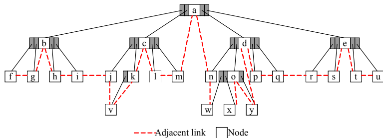
Fig.3 BATON*-tree structure
