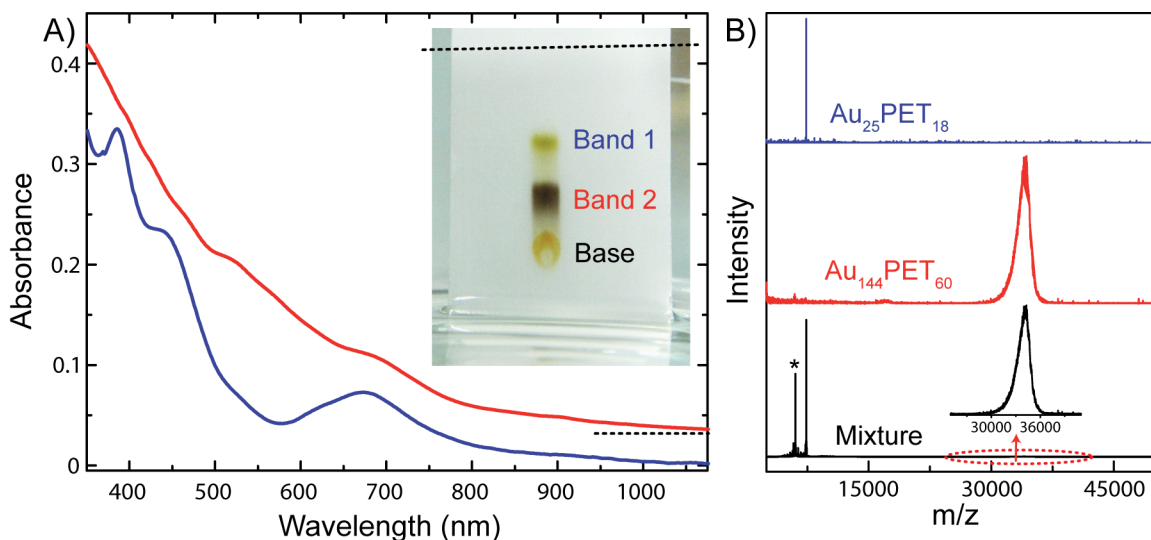
Figure 2. A) UV-vis spectra of the two bands separated by TLC. Red trace matches well with the previously reported UV-vis spectrum of Au 144 PET 60 cluster 15 and blue trace matches with the UV-vis spectrum of Au 25 PET 18 cluster. 11 The red trace has been vertically shifted for clarity. Inset: Photograph of the TLC plate used for cluster separation (solvent front marked as a dashed line). B) MALDI MS data of crude (black trace) and isolated clusters (blue and red trace) confirming that bands 1 and 2 consist of isolated Au 25 PET 18 and Au 144 PET 60 , respectively. The fragmented product, Au 21 L 14 is shown with an asterisk (*).
