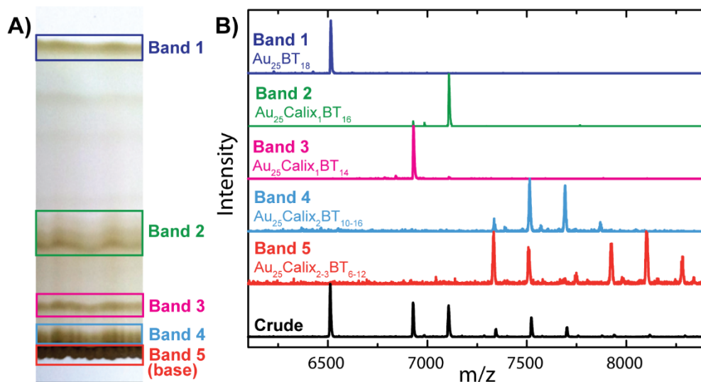
Figure 4. A) Photograph of the TLC plate used for cluster separation. The faint bands observed between bands 1 and 2 are caused by sticking of the clusters to the TLC plate upon drying between runs (Note that the TLC plates were eluted repeatedly. See also supporting information, Figure S-4). B) MALDI MS data of \text{Au}_{25}\text{Calix}_{0-3}\text{BT}_{6-18} crude product before TLC (black trace) and bands 1-5 separated by TLC.
