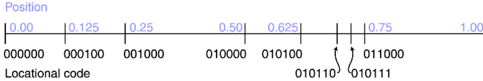
Figure 1. A 1D spatial partitioning over [0,1] showing the relationship between the position of the cell's left corner and the cell's locational code.
