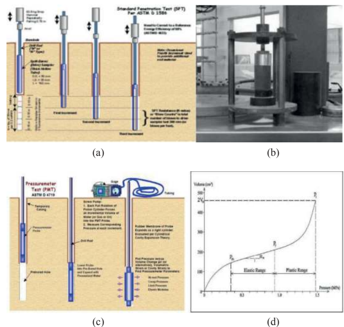
Fig. 1 Diagrams depicting the principles of the (a) SPT test, (b) UCS test, (c) Pressuremeter test and (d) a typical pressuremeter graph.
