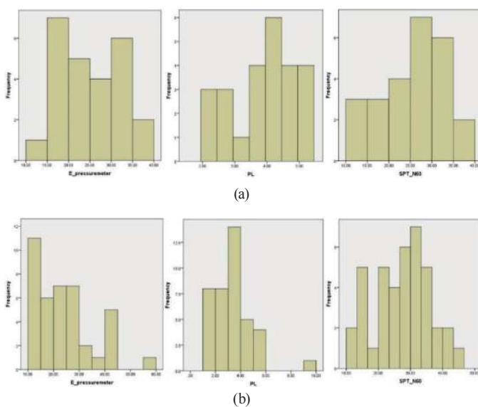
Fig. 3 Histograms of the in situ test data (a) sandy soil and (b) clayey soil (pressuremeter modulus ( E_M ), limit pressure ( P_L ) and corrected SPT blow count ( N_{60} ))
