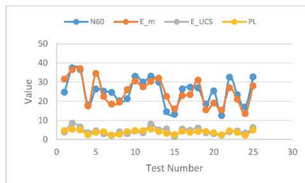
Fig. 7 Trending graph of the correlated parameters in sandy soils
