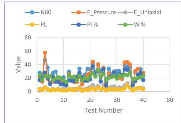
Fig. 10 Trending graph of the correlated parameters in clayey soils
