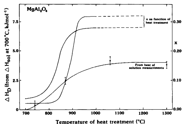
Fig. 5. Degree of disorder ( x ) versus temperature of heat treatment ( ^\circ\text{C} ) for two natural samples of \text{MgAl}_2\text{O}_4 from Schmocker and Waldner (1976), and the change in heat of solution with temperature of heat treatment for another natural sample of \text{MgAl}_2\text{O}_4 from Navrotsky and Kleppa (1967). Note the similarity in the forms of the curves.
