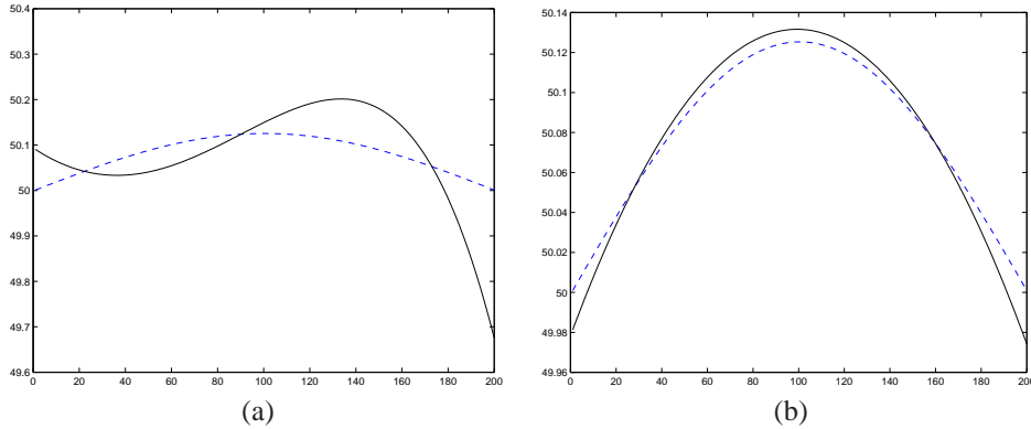
FIGURE 4.1. Example 4.1: Computed approximate solutions \mathbf{x}_k determined by RR-GMRES using the discrepancy principle. The dashed curves show the vector \hat{\mathbf{x}} ; the continuous curves display in (a) the iterate \mathbf{x}_3 determined without regularization operator ( L := I ), and in (b) the iterate \mathbf{x}_0 determined with the regularization operator L := L_{3,0} .
