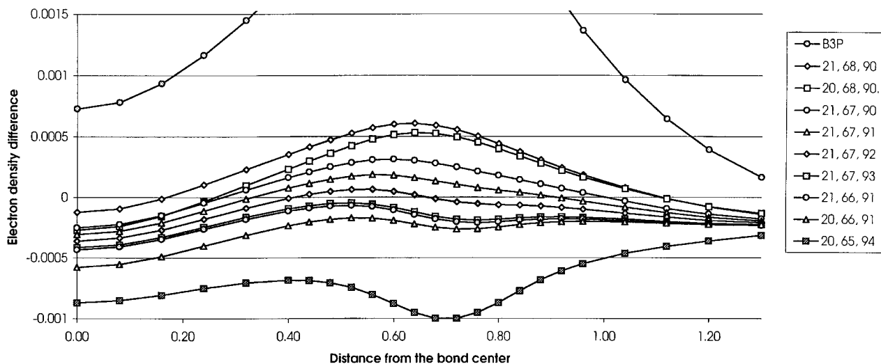
FIGURE 5. Electron density differences (a.u.) calculated at an experimental H_2 distance as a function of the distance (Bohrs) from the bond center in H_2 along the internuclear axis. The CISD/6-311G(d, 2pd) electron density was used as a reference. Negative values indicate smaller electron densities compared with CISD results. The legend shows 100-fold values of A , B , and C . Numbers 21, 68, 90 indicate A = 0.21 , B = 0.67 , and C = 0.91 in eq. (1).
