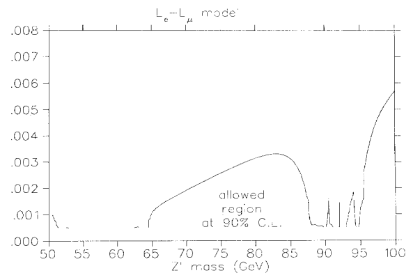
FIG. 2. The allowed region at 90% C.L. in (g'_1, M_{Z'_1}) space for the gauged L_e - L_\mu model.
