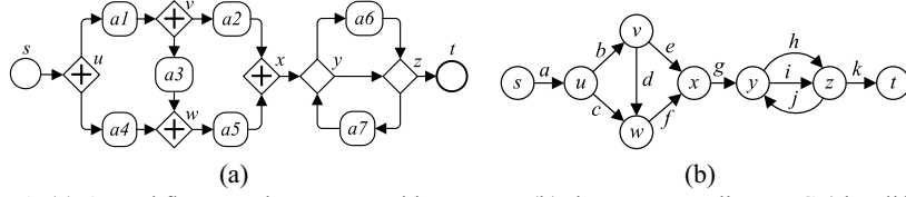
Fig. 1. (a) A workflow graph represented in BPMN, (b) the corresponding TTG (simplified)
