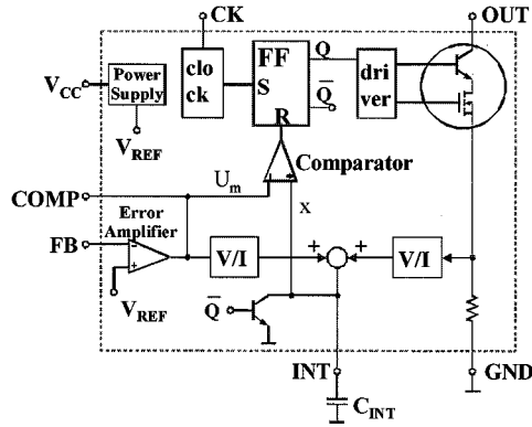
Fig. 5. Possible smart power integration scheme.
