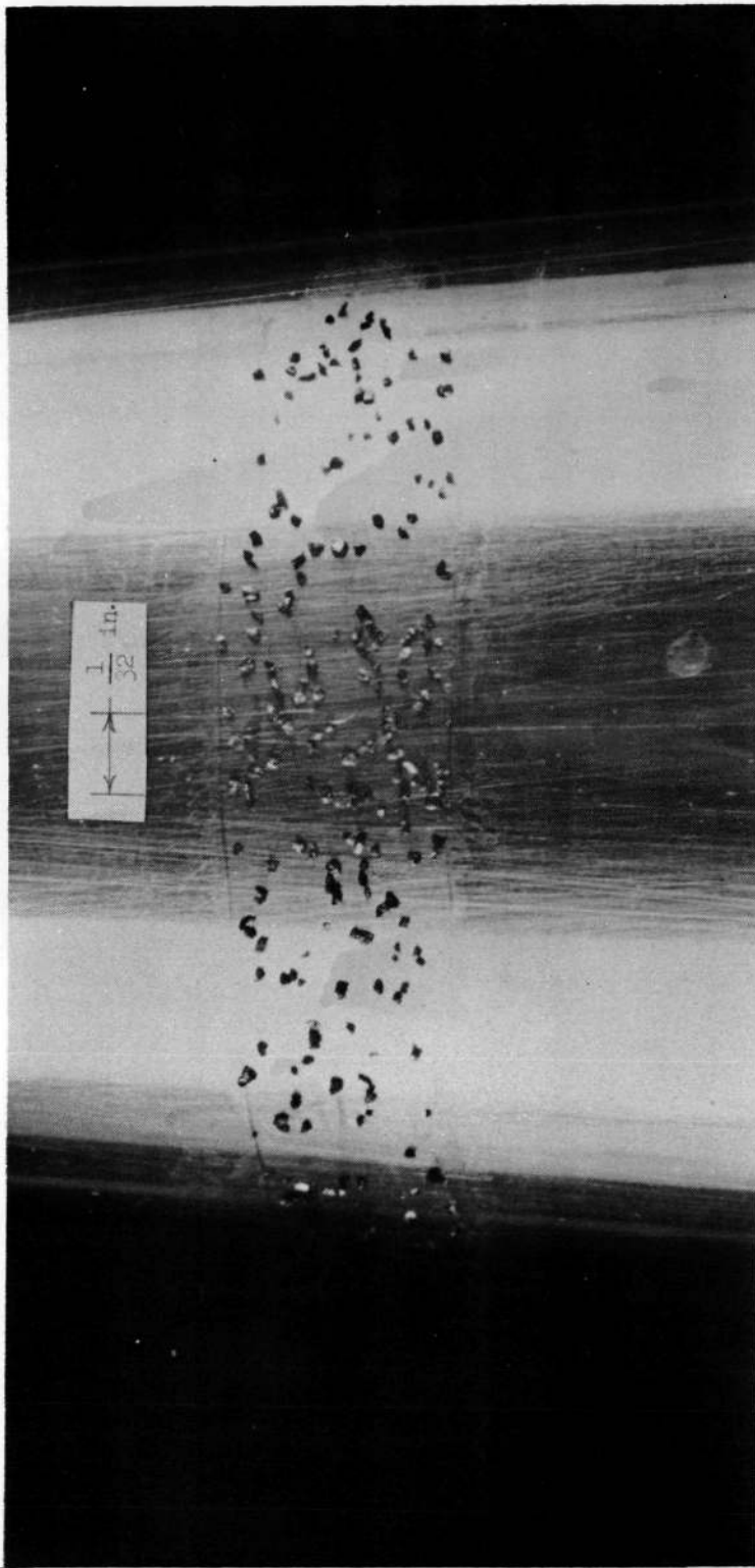
(b) No. 80 carborundum grains. L-57-4945.1
