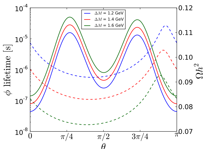
Figure 9. The lifetime of \phi^\pm (dashed) and the DM relic density \Omega h^2 (solid) as functions of the L-R mixing parameter \theta . The DM mass is fixed at 300 GeV and \Delta M is varied as 1.2 (blue), 1.4 (red) and 1.6 (green) GeV.
