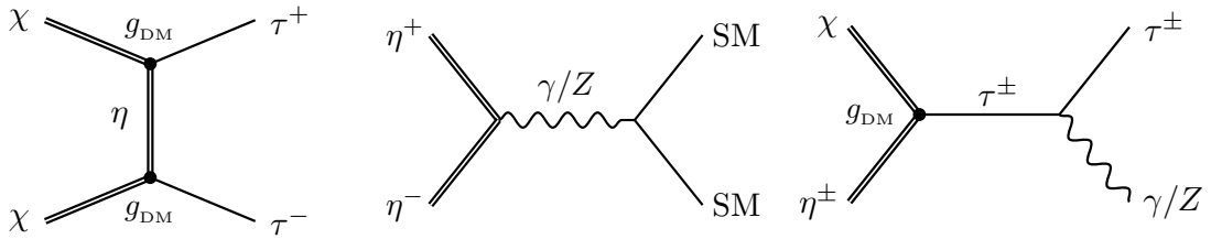
Figure 1. Annihilation and co-annihilation processes.
