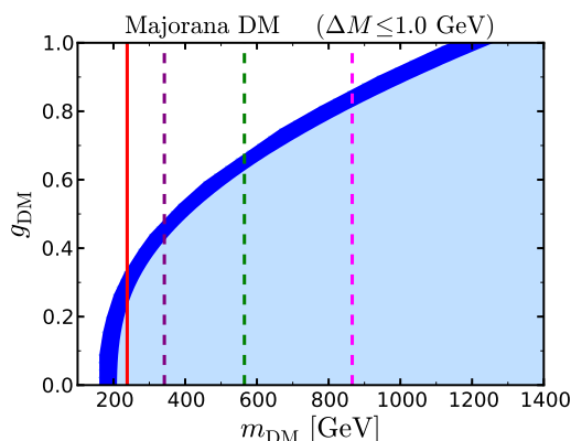
Figure 7. Model 1a: plot of the coupling g_{\text{DM}} versus the dark matter mass m_{\text{DM}} = m_\chi . We scan over \Delta M \leq 1 \text{ GeV} , where \Delta M = M_\phi - m_\chi , this is the mass region where the HSCP limits are independent of the coupling g_{\text{DM}} . The dark blue band satisfies the correct DM relic abundance within 3\sigma , the region in light blue overproduces the amount of DM. The colour-coding for the exclusion regions is the same as in the previous figure.
