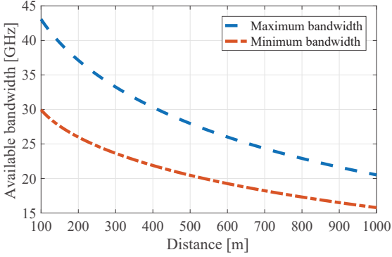
Fig. 4. The estimated available bandwidth based on one sided three dB loss (minimum bandwidth) and the maximum bandwidth allowed by the full transmission window.
