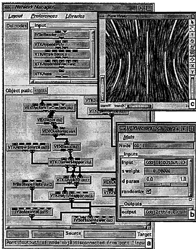
Figure 12: Clustering pipeline and visualization in the VISION system
