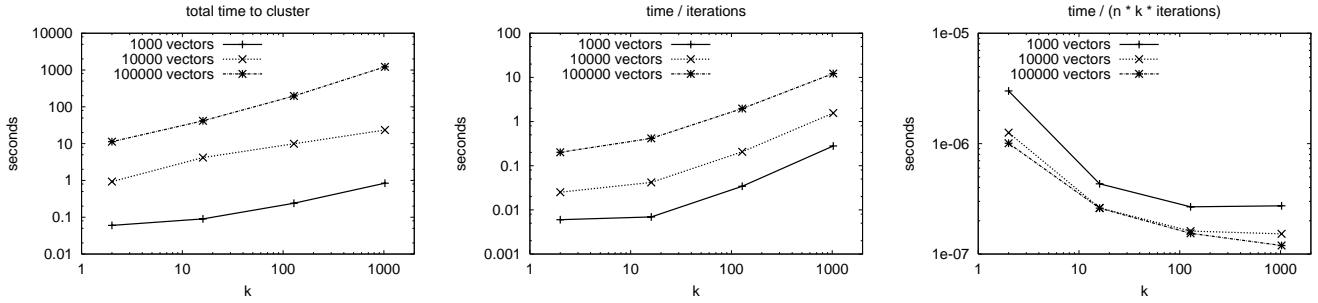
Figure 1: These plots show how varying the number of vectors and clusters affects the amount of time required to cluster with SimPoint 3.0. For this experiment we generated uniformly random data in 15 dimensions. The first plot shows total time, the second plot shows the time normalized by the number of iterations performed, and the third plot shows the time normalized by the number of operations performed. Both the number of vectors and the number of clusters have a linear influence on the run-time of k -means.
