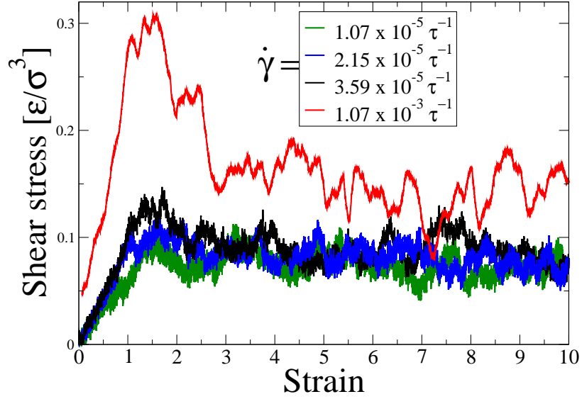
Figure 5.2: Stress response for \dot{\gamma} = 1.07 \times 10^{-5} \tau^{-1} , 2.1 \times 10^{-5} \tau^{-1} , 3.59 \times 10^{-5} \tau^{-1} , 1.07 \times 10^{-3} \tau^{-1} .
