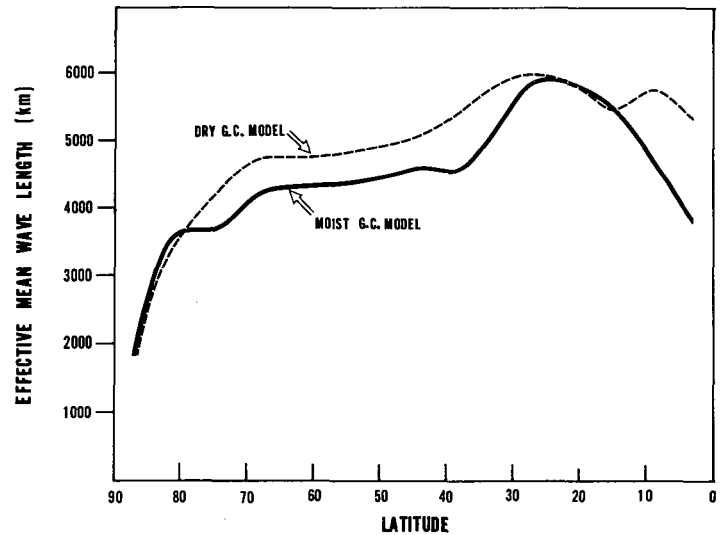
FIGURE 8.4.—Latitudinal distributions of the pressure-weighted vertical mean of the effective wavelength ( 2\pi a \cos \theta / \bar{n} , where \theta is latitude and a the radius of the earth) for both the moist and the dry atmosphere.
