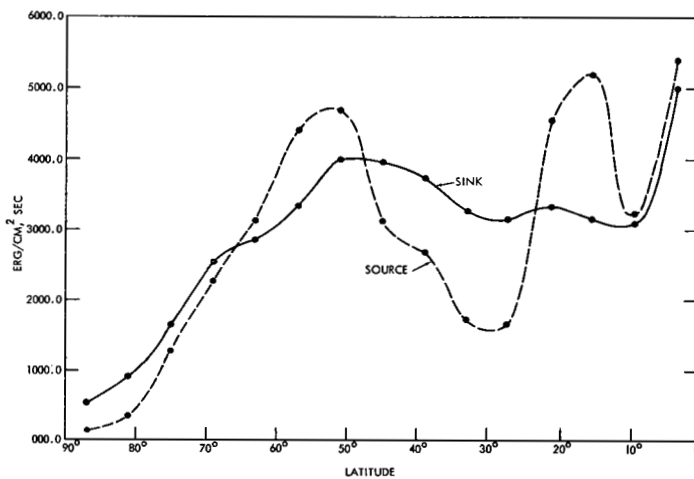
FIGURE 9.4.—The latitudinal distributions of source ( -\overline{\mathbf{V} \cdot \nabla \phi} ) and sink ( \overline{\mathbf{V} \cdot \mathbf{F}} ) of kinetic energy in the model atmosphere.
