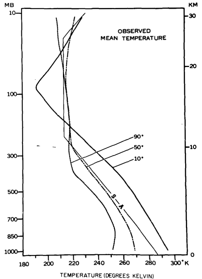
FIGURE 5.2.—In the left and right hand sides of the figure are shown the vertical distribution of computed and observed temperature at various latitudes.
