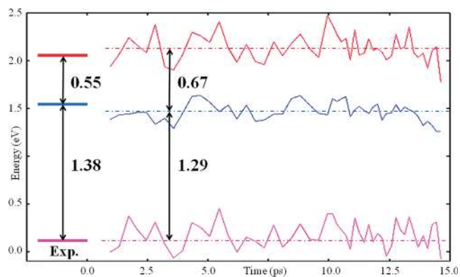
Figure 3. Time (ps) evolution of the excited state oxidation potential (red), TiO 2 -based LUMO (blue), and dye-based HOMO (magenta) energies in eV. The zero of the energy scale is set to the value of the HOMO energy of the starting configuration. Dashed lines represent average values of the three quantities. Also shown on the left are experimental spectro-electrochemical data from refs 10 and 32.
