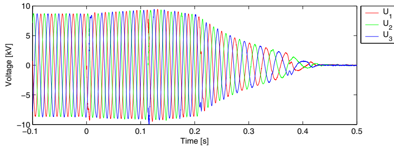
Figure 59: Line to neutral voltages U_{10wt2} measured at the 10 kV connection point of wind turbine #2.
