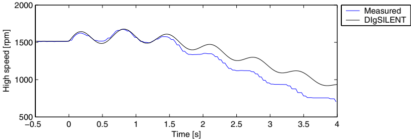
Figure 80: Measured and simulated (DIgSILENT) generator speed of wind turbine #1.
