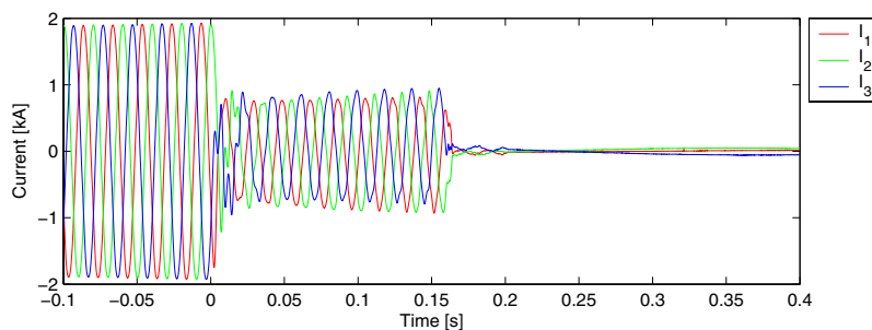
Figure 28: Generator line currents I_{gen} of the generator of wind turbine #1.
