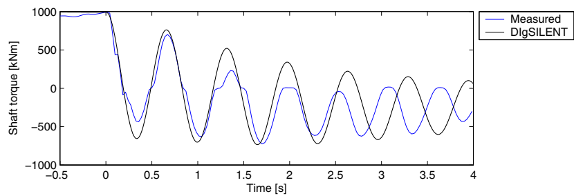
Figure 92: Measured and simulated (DIgSILENT) shaft torque of wind turbine #1.
