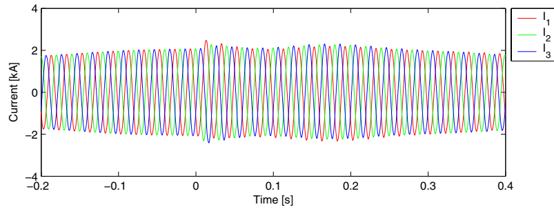
Figure 67: Measured line currents I_{gen} of the generator of wind turbine #1.
