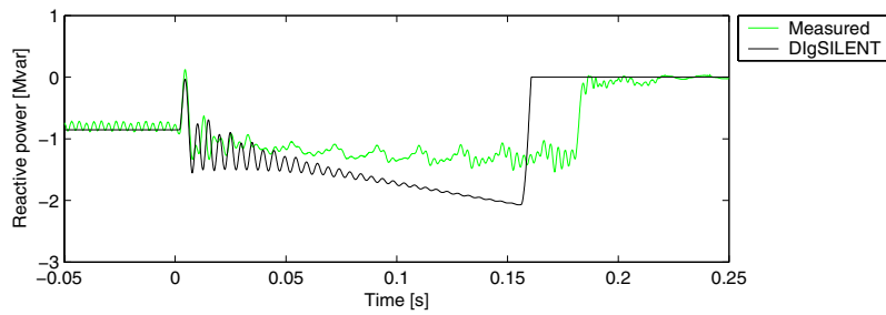
Figure 88: Measured and simulated (DIgSILENT) generator reactive power of wind turbine #1.
