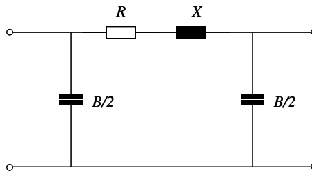
Figure 2. Single line diagram for cable
