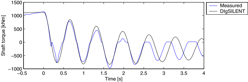
Figure 81: Measured and simulated (DIgSILENT) shaft torque of wind turbine #1.
