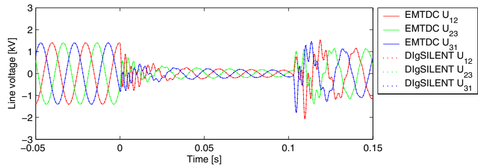
Figure 13: Simulated generator voltages with EMTDC and DIgSILENT
