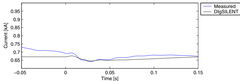
Figure 116: Positive sequence of measured and simulated (DIgSILENT) generator currents I_{gen} of wind turbine #1.
