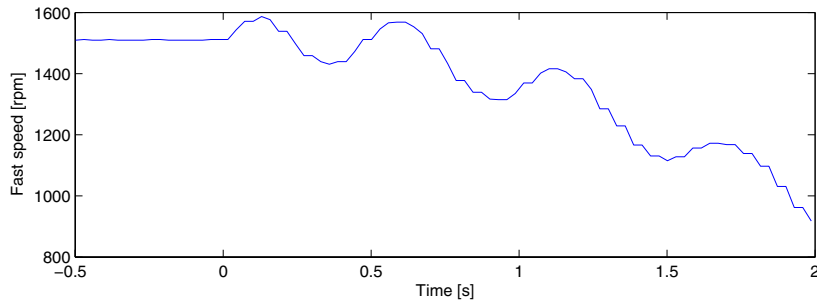
Figure 50: Generator speed of wind turbine #1.
