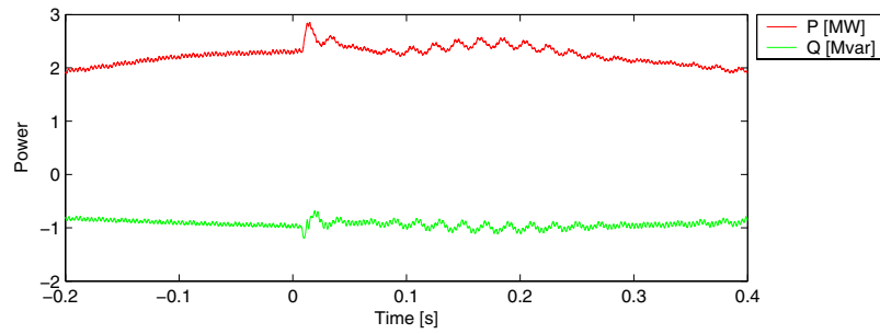
Figure 68: Active power P_{gen} and reactive power Q_{gen} of the generator of wind turbine #1.
