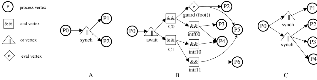
Figure 3: DSDG Examples.
