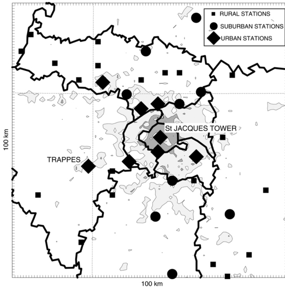
Figure 1. Meteo-France observational network in the Paris area. The extent of urbanization defined by the model is represented: Light grey = 50\% < \text{urbanization} < 80\% and dark grey = urbanization > 80\% .
