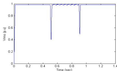
Figure-21. Voltage V_{rms} at load point: With DVR Energy Storage of 7kv.
