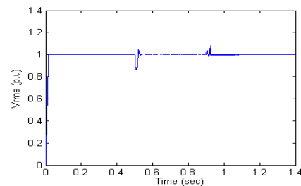
Figure-17. Voltage V_{rms} at the load point: with Energy Storage of 40.7kv
