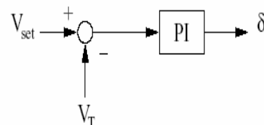
Figure-3. Indirect PI controller.
