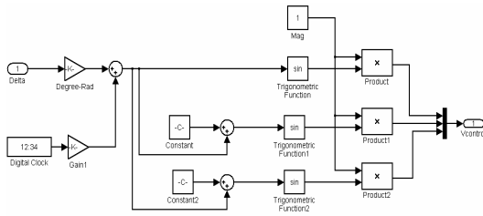
Figure-4. Phase-Modulation of the control angle \delta .
