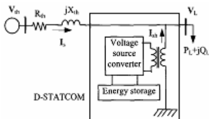
Figure-10. Schematic diagram of a D-STATCOM.
