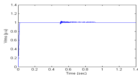
Figure-19. Voltage V_{rms} at the load point: with D-STATCOM Energy Storage of 16.8kv
