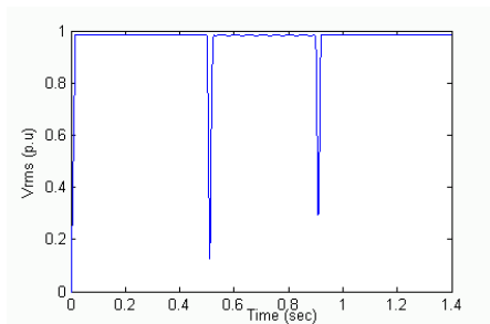
Figure-25. Voltage V_{rms} at the load point: with DVR Energy Storage of 4.9kv.
