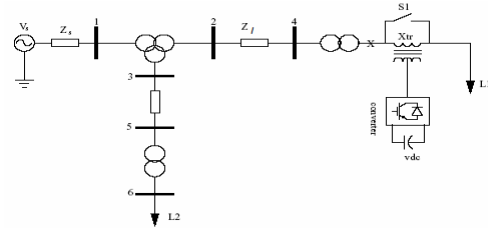
Figure-7. Single line diagram of the test system for DVR.
