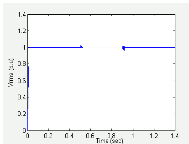
Figure-15. Voltage V_{rms} at the load point: with D-STATCOM Energy Storage of 20.9kv
