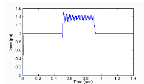
Figure-18. Voltage V_{rms} at the load point: Without D-STATCOM.
