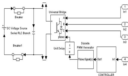
Figure-9. Simulink model of DVR.
