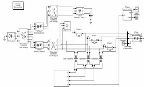
Figure-8. Simulink model of DVR test system for voltage sag.
