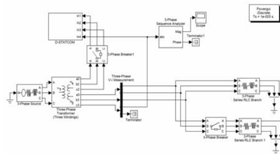
Figure-12. Simulink model of D-STATCOM test system.
