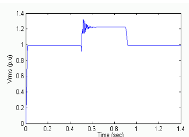
Figure-22. Voltage V_{rms} at the load point: without DVR.
