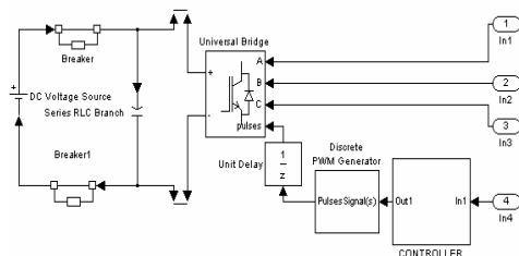
Figure-13. Simulink model of D-STATCOM.
