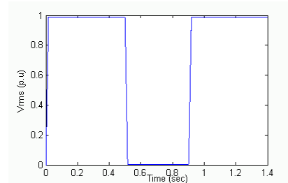
Figure-16. Voltage V_{rms} at the load point: without D-STATCOM.
