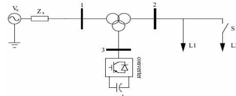
Figure-11. Single line diagram of the test system for D-STATCOM.
