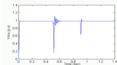
Figure-23. Voltage V_{rms} at the load point: with DVR Energy Storage 6.8kv.
