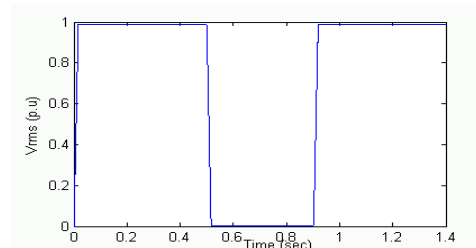
Figure-24. Voltage V_{rms} at the load point: without DVR. When the DVR is in operation the voltage sag is mitigated almost completely, and the rms voltage at the sensitive load point is maintained at 98%, as shown in Figure-25.
