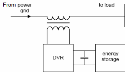
Figure-1. Example of a standard configuration for a DVR.
