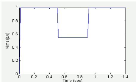
Figure-14. Voltage V_{rms} at the load point: without D-STATCOM.
