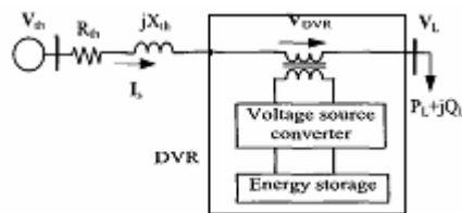
Figure-2. Schematic diagram of a DVR
