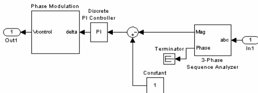
Figure-5. Simulink model of DVR Controller.
