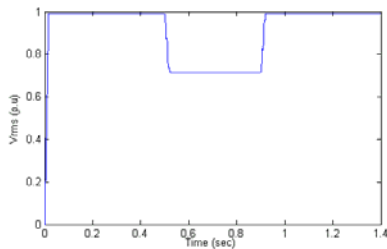
Figure-20. Voltage V_{rms} at load point: without DVR.
