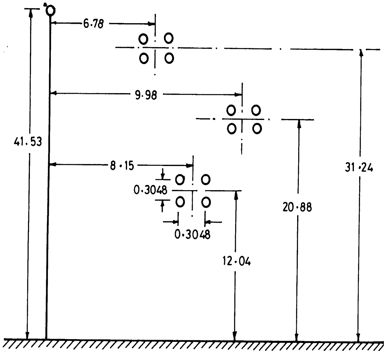
Fig. 1: 400 kV Transmission line (conductor spacing in metres) Upper : Phase a Middle : Phase b Lower : Phase c
