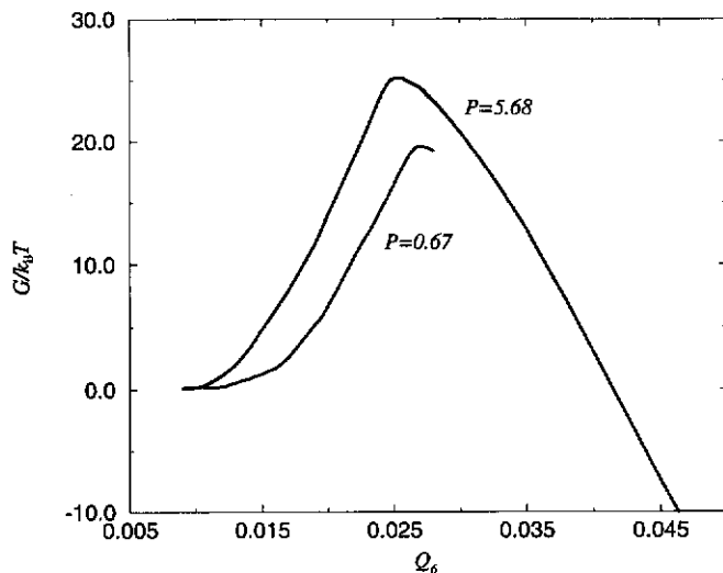
Fig. 4 Gibbs free energy of a Lennard-Jones system as a function of crystallinity ( Q_6 ) at 20% supercooling for two different pressures, i.e. P = 5.68 ( T = 0.92 ) and P = 0.67 ( T = 0.6 ). The Gibbs free energy barriers are ca. 25.1k_B T at P = 5.68 and 19.4k_B T at P = 0.67 .
