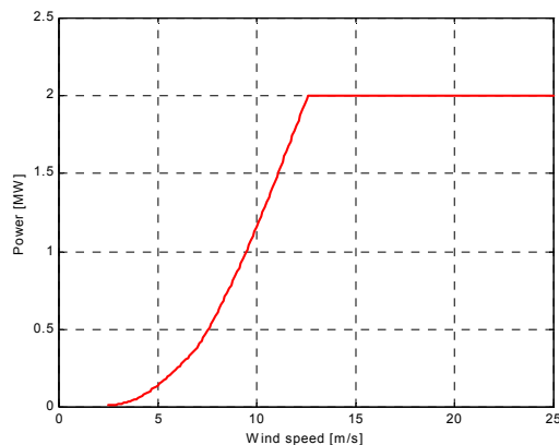
Figure 27. Simulated power curve used to fit the wind speeds for the simulations.
