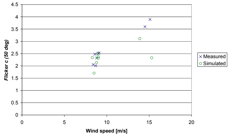
Figure 42. Measured and simulated flicker coefficients for continuous operation of wind turbine 1. Grid impedance angle 50 deg.
