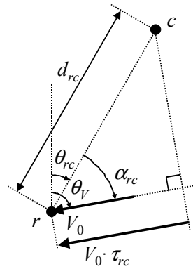
Figure 22. Two points r and c each corresponding to a wind turbine. The distance between the two points r and c is d_{rc} , with a direction \theta_{rc} from north. V_0 is the mean wind speed, and \theta_V is the wind direction. \alpha_{rc} is the resulting inflow angle, and \tau_{rc} is the delay time.
