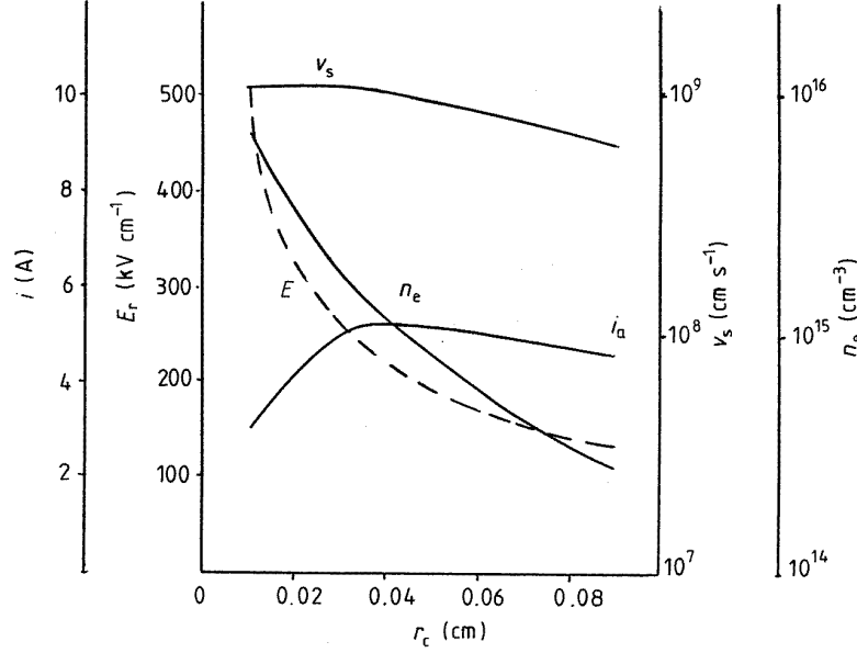
Figure 2. The peak values of the streamer velocity, electric field and electron density at the streamer head, and conduction current through the anode versus r_c . The curves correspond to the same initial conditions as those given in figure 1.
