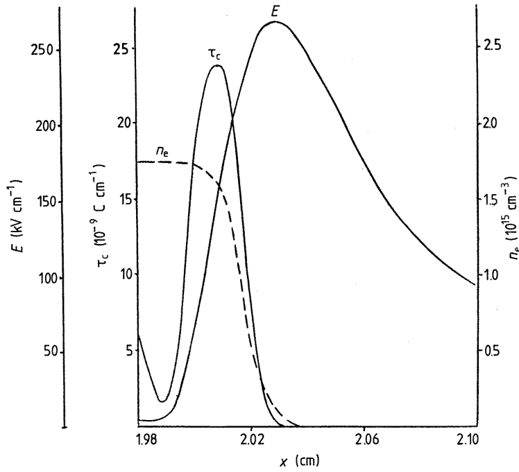
Figure 1. Axial profiles of E , \tau_c and n_e at the streamer head at 3.95 ns. The initial conditions used are a spherical anode of radius R_a = 1 cm, the applied voltage of 100 kV and the fixed radius r_c = 0.03 cm.
