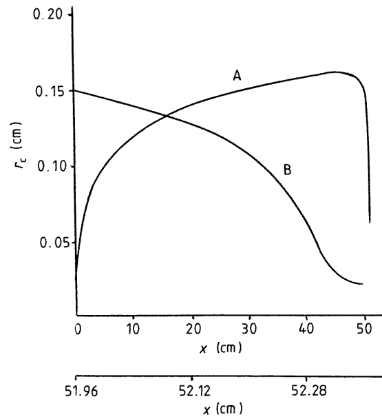
Figure 14. The axial profile of r_c for E_0 = 15 \text{ kV cm}^{-1} at 98 ns (curve A, upper abscissa). Curve B and the lower abscissa show a more accurate representation of this profile at the streamer head.
