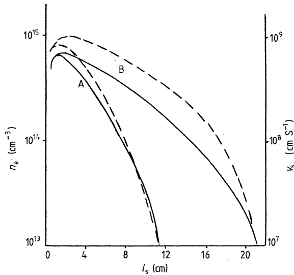
Figure 3. The maximal electron density in the streamer channel (broken curves) and the streamer velocity (full curves) calculated for the simple ionic kinetics with \beta_{ei} = 2 \times 10^{-6} \text{ cm}^3 \text{ s}^{-1} (curve A) and 2 \times 10^{-7} \text{ cm}^3 \text{ s}^{-1} (curve B). The curves correspond to the same initial conditions as those given in figure 1.
