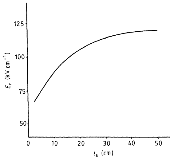
Figure 10. The peak electric field at the streamer head versus the streamer length at E_0 = 15 \text{ kV cm}^{-1} .
