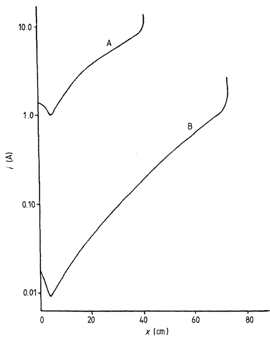
Figure 13. Axial profiles of the conduction current for E_0 = 10 \text{ kV cm}^{-1} at 90.2 ns (curve A) and for E_0 = 15 \text{ kV cm}^{-1} at 545 ns (curve B).
