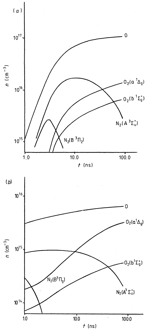
Figure 5. The time evolution of densities of O, O_2(a^1\Delta_g) , O_2(b^1\Sigma_g^+) , N_2(A^3\Sigma_u^+) and N_2(B^3\Pi_g) in the streamer plasma (a) near the anode and (b) at a distance of 5.1 cm from it. The curves correspond to the same initial conditions as those given in figure 1.
