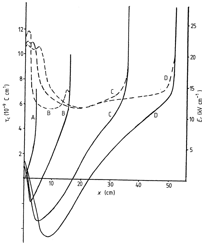
Figure 11. Axial profiles of \tau_c (full curves) and E_c (broken curves) for E_0 = 15 \text{ kV cm}^{-1} at 40 ns (curve A), 65 ns (curve B), 85 ns (curve C) and 98 ns (curve D).
