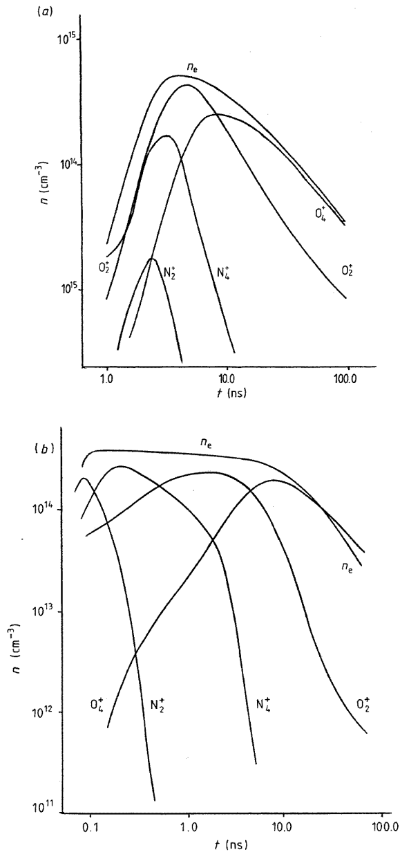
Figure 4. The time evolution of densities of electrons, O_2^+ , O_4^+ , N_2^+ and N_4^+ in the streamer plasma (a) near the anode and (b) at a distance of 5.1 cm from it. The curves correspond to the same initial conditions as those given in figure 1.
