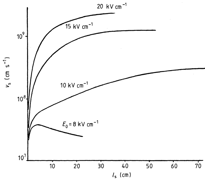
Figure 9. v_c versus the streamer length at different values of E_0 .
