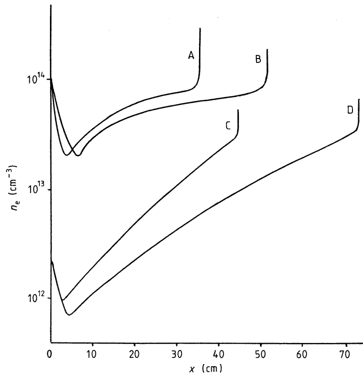
Figure 12. Axial profiles of n_e for E_0 = 15 \text{ kV cm}^{-1} at 85 ns (curve A) and 98 ns (curve B) and for E_0 = 10 \text{ kV cm}^{-1} at 442 ns (curve C) and 545 ns (curve D).
