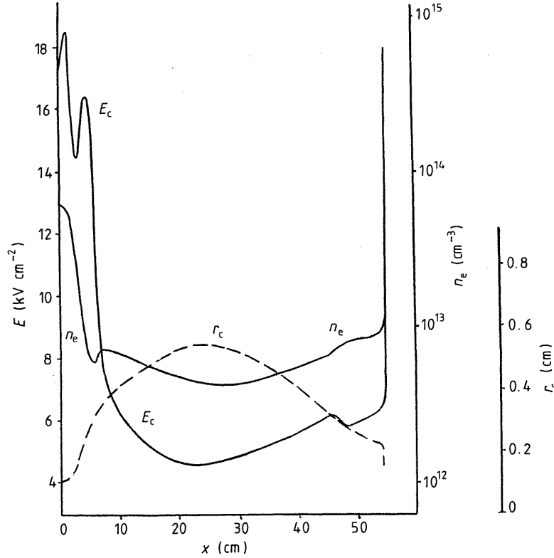
Figure 8. Axial profiles of r_c , E_c and n_e at 138 ns. The curves correspond to the same initial conditions as those given in figure 6.
