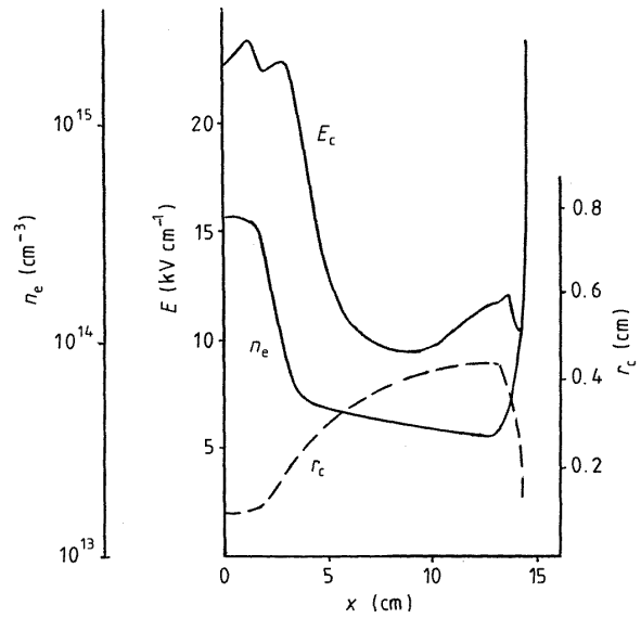
Figure 6. Axial profiles of r_c , n_e and E_c at the instant at which the total anode current peaks ( t = 39.3 \text{ ns} ). Initial conditions used were a spherical anode with R_a = 12.5 \text{ cm} and applied electric field strength near the anode of 40 \text{ kV cm}^{-1} .
