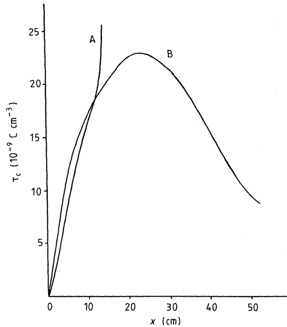
Figure 7. Axial profiles of \tau_c at 39.3 ns (curve A) and 138 ns (curve B). The curves correspond to the same initial conditions as those given in figure 6.
