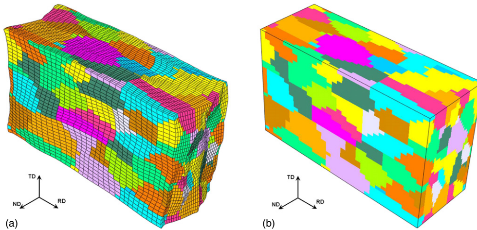
Figure 3. Deformed configuration of the RVE from rolling simulations after 40% thickness reduction; (a) FE and (b) FFT.
