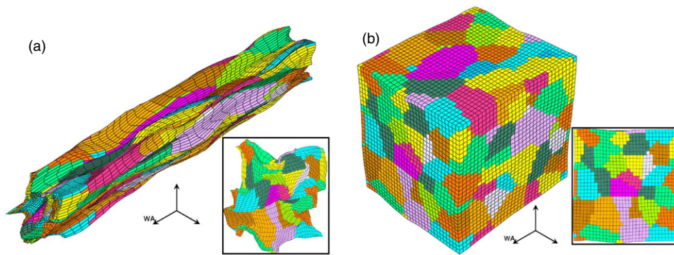
Figure 5. Deformed configuration of the RVE calculated with FE in the wire drawing case—(a) after 50% diameter reduction, (b) after 10% equivalent strain (Inset—cross sectional views).
