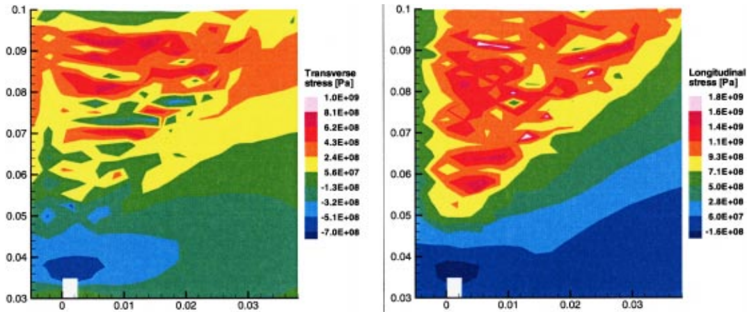
Fig. 9 Transverse residual stress and longitudinal residual stress for welds in upper groove. Distance in m.
