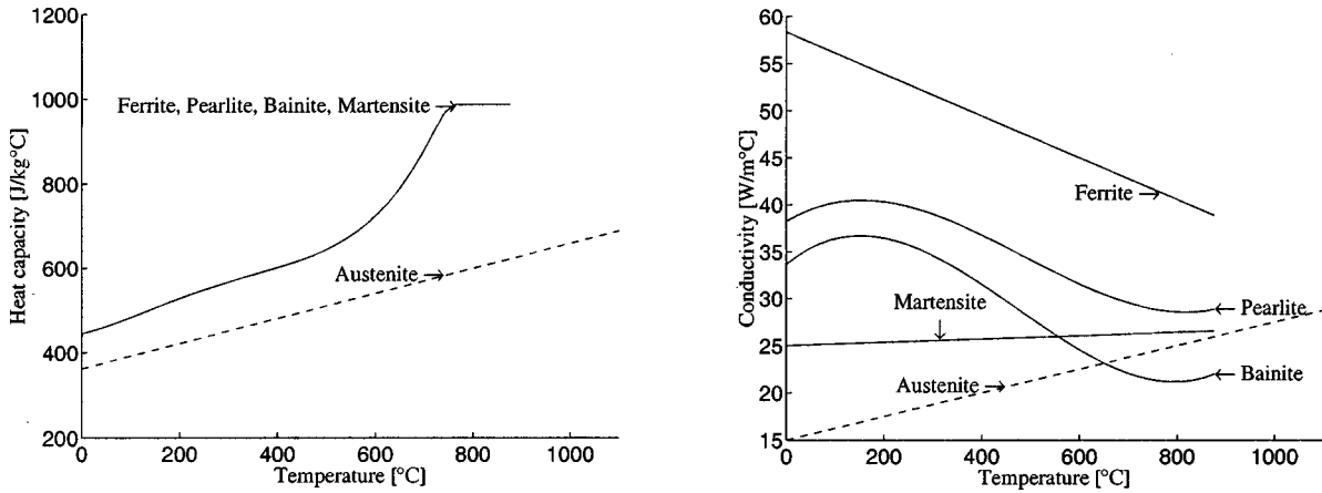
Fig. 2 Thermal properties assigned to each phase
