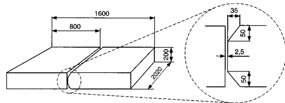
Fig. 6 Geometry of the plates and the groove, distances in mm
