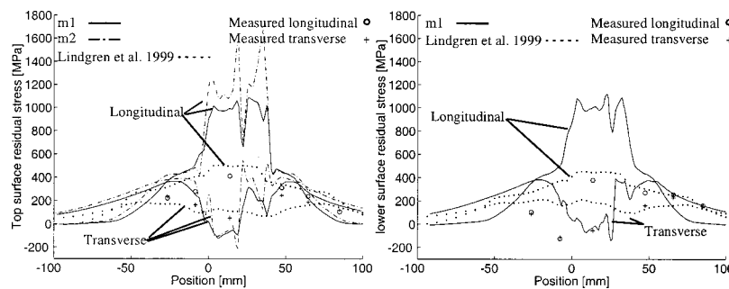
Fig. 10 Calculated and measured residual stress at the top and bottom surfaces. The origin ( x=0 ) is placed at the left side of the joint.
