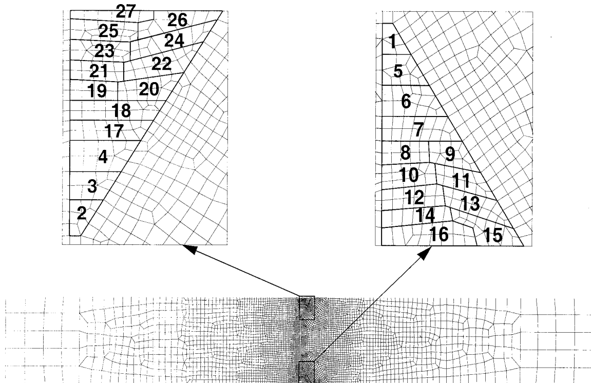
Fig. 7 The mesh and corresponding weldpasses
