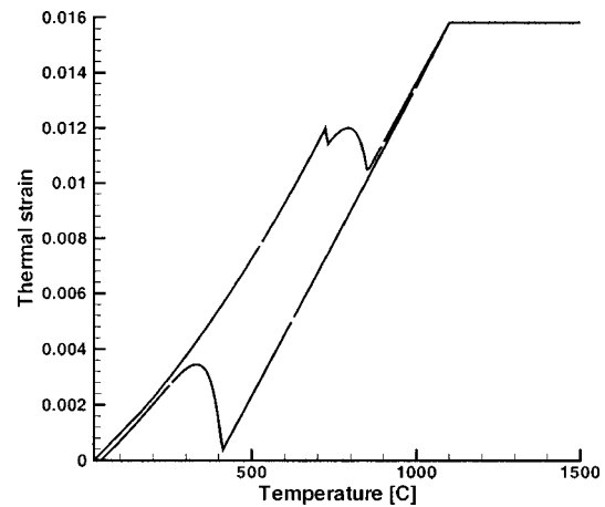
Fig. 4 Computed thermal strain as a function of temperature
