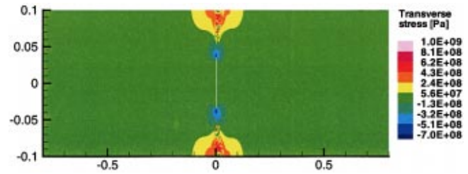
Fig. 8 Transverse residual stress for a part of the plate. Distance in m.
