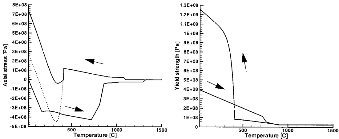
Fig. 5 Computed axial stress with transformation plasticity (solid line) and without transformation plasticity (dashed line) and computed virgin yield strength as a function of temperature
