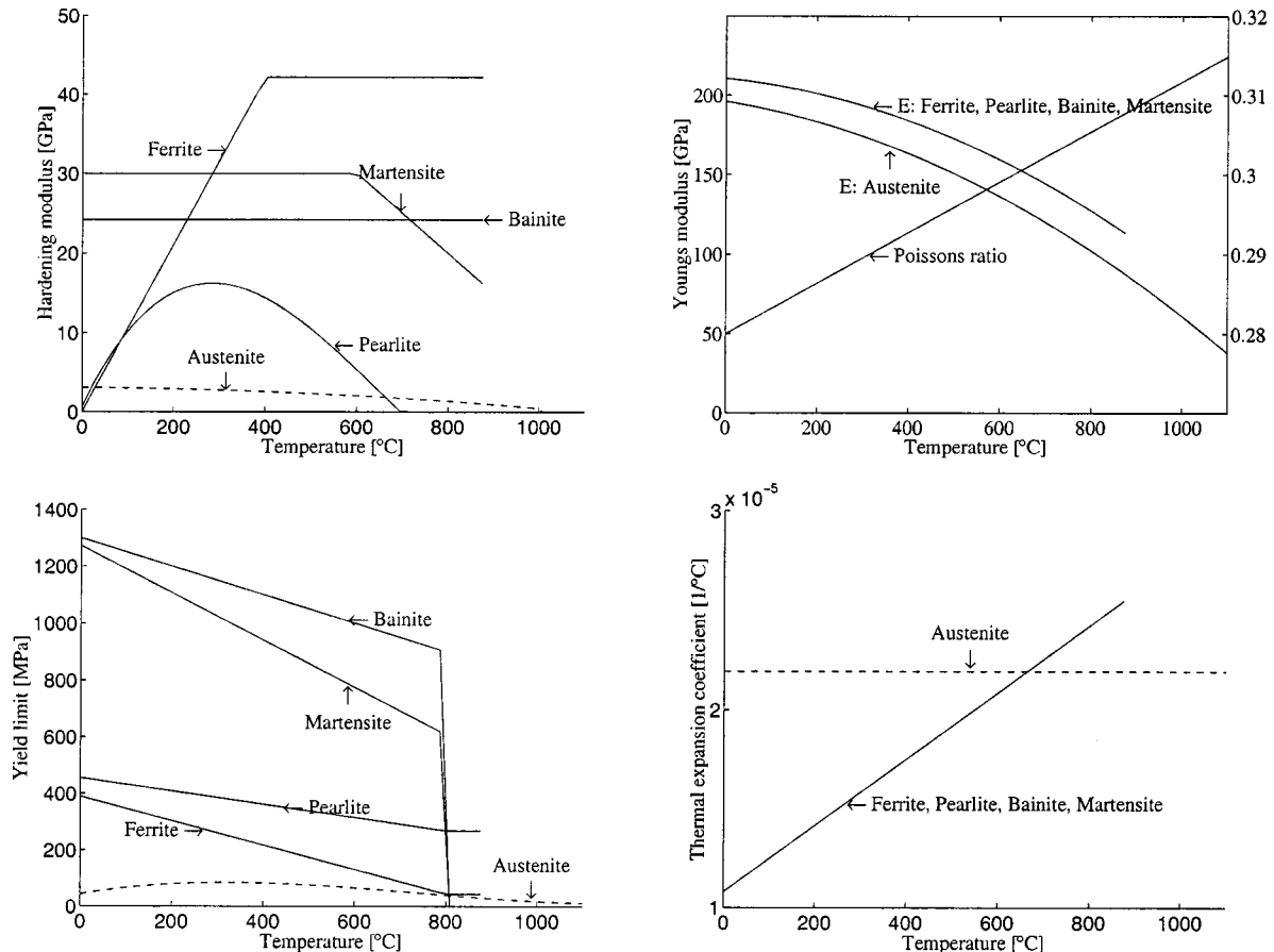
Fig. 3 Mechanical properties assigned to each phase
