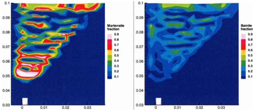
Fig. 11 Final martensite and bainite fractions for welds in upper groove
