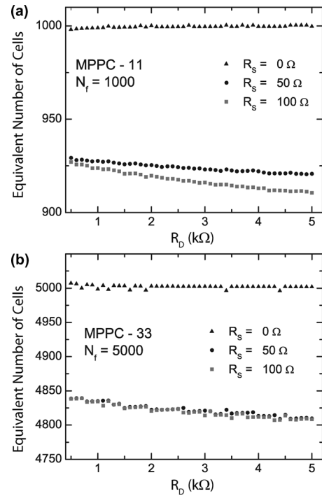
Fig. 6. Equivalent number of fired cells N_f^e obtained from the simulated data, for a true number of fired cells N_f = 1000 for MPPC-11(a) and for N_f = 5000 for MPPC-33 (b), as a function of R_D .
