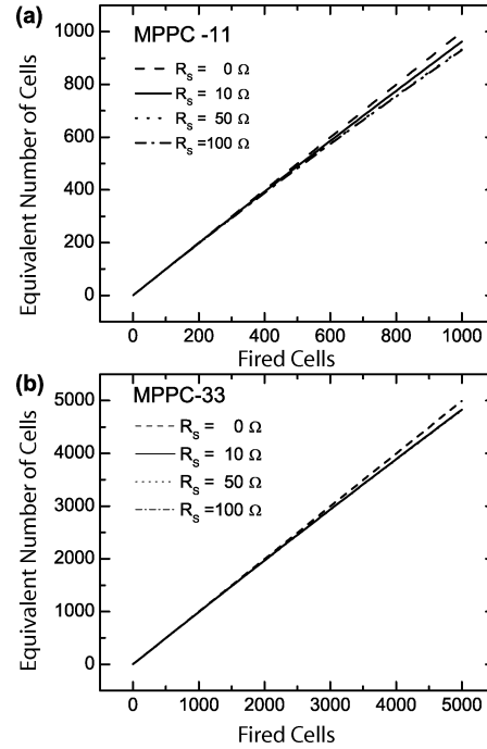
Fig. 9. Predicted SiPM signal, normalized to the single cell charge, as a function of the true number of fired cells, for (a) MPPC-11 and (b) MPPC-33. Both SiPMs show an increasing deviation of the equivalent number of fired cells from the true value of N_f with increasing N_f . Please note that the lines for R_S = 50 \Omega and R_S = 100 \Omega overlap in both figures.
