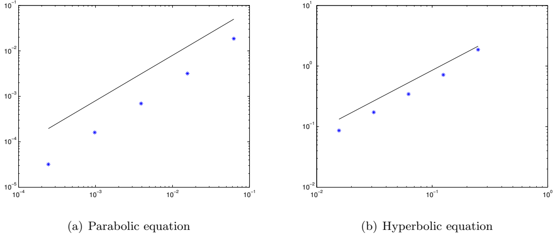
FIGURE 2. Simulated errors with respect to the time discretization and a line as reference slope on a logarithmic scale.
