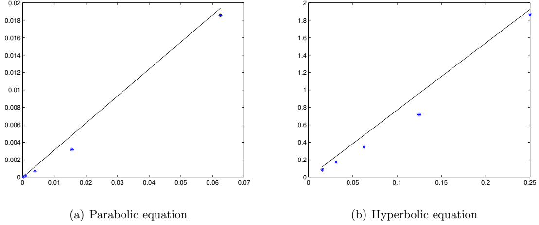
FIGURE 3. Simulated errors with respect to the time discretization and a line as reference slope on a linear scale.
