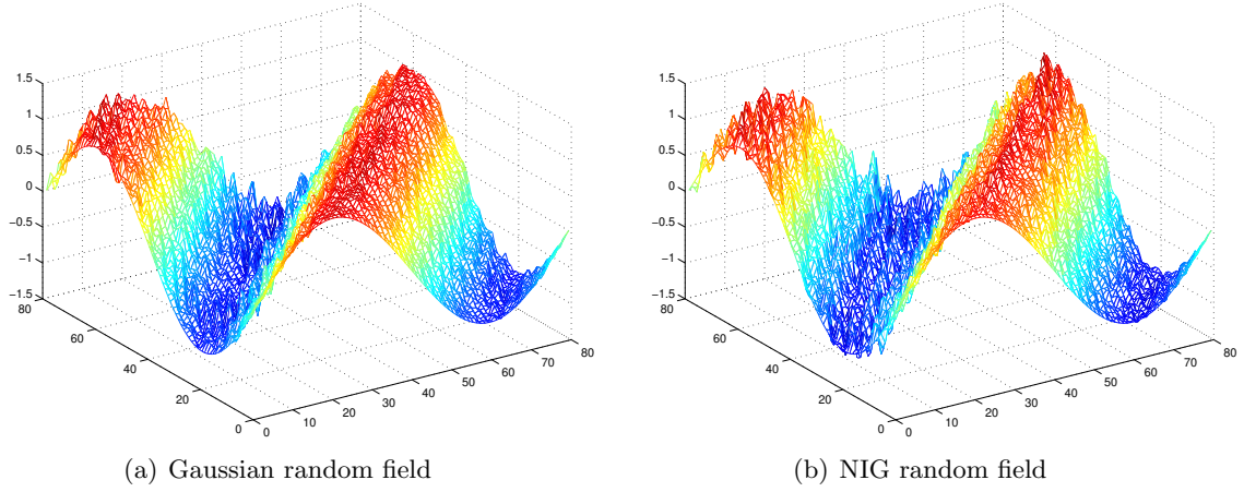
FIGURE 4. Simulation of one path of a hyperbolic equation with additive noise on a grid with 80 \times 80 points.
