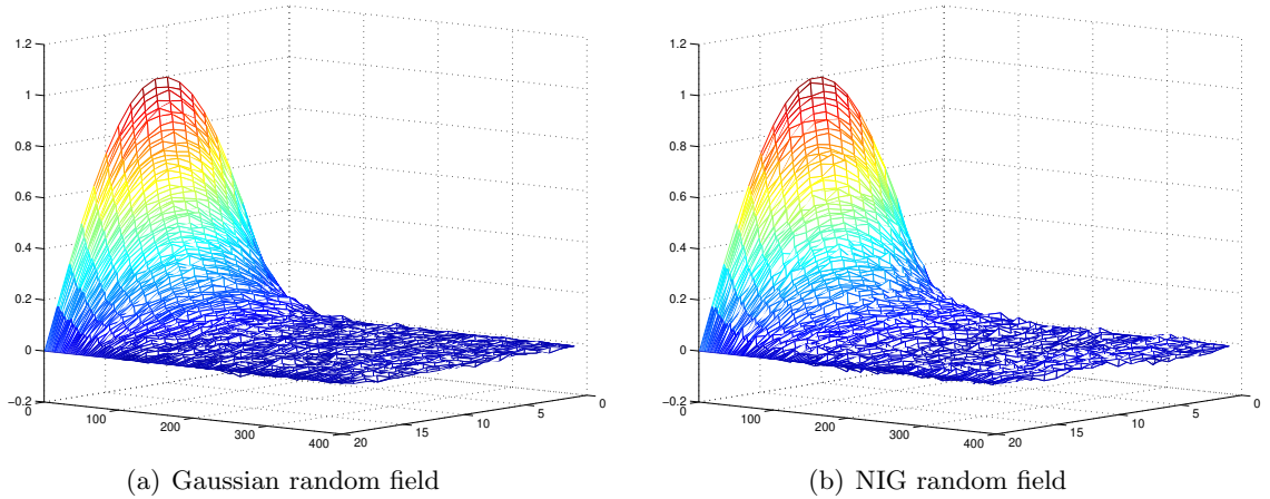
FIGURE 1. Simulation of one path of a heat equation with additive noise on a grid with 400 \times 20 points.
