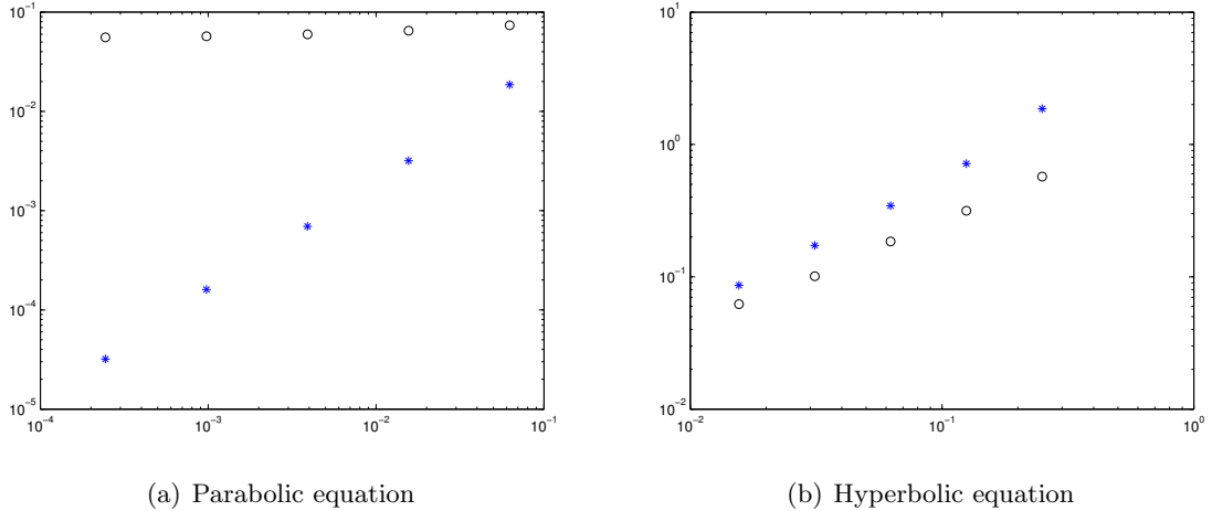
FIGURE 5. Simulated errors with respect to the time discretization for different kernel functions on a logarithmic scale.
