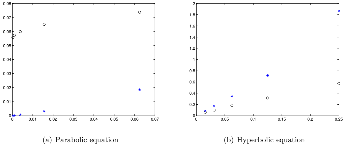
FIGURE 6. Simulated errors with respect to the time discretization for different kernel functions on a linear scale.
