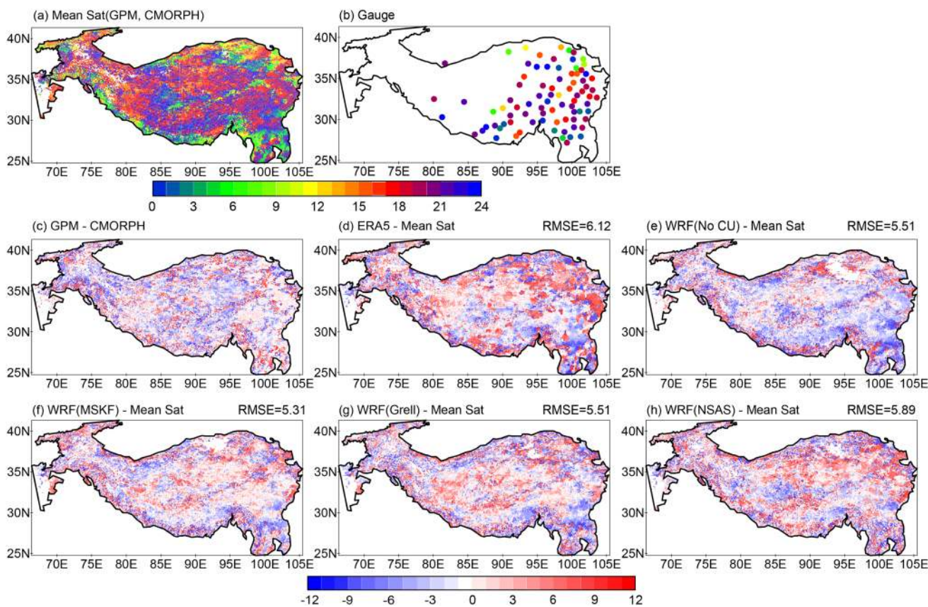
Fig. 6 Same as Fig. 4, but for precipitation intensity (precipitation rate ( \text{mm h}^{-1} ) averaged over all the hours when hourly precipitation \geq 0.1 \text{ mm h}^{-1} )
