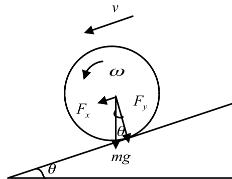
Fig. 1 single-wheel on hill road dynamics mode
