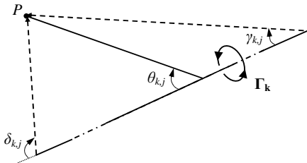
Figure 7: Integration angles - Branch j of the horseshoe vortex k
