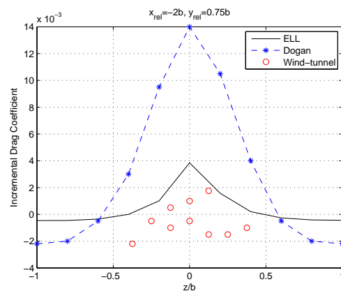
Figure 22: Variations of the incremental drag coefficient with vertical spacing
