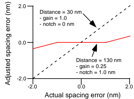
Figure 3: Gain and notch filtering.
