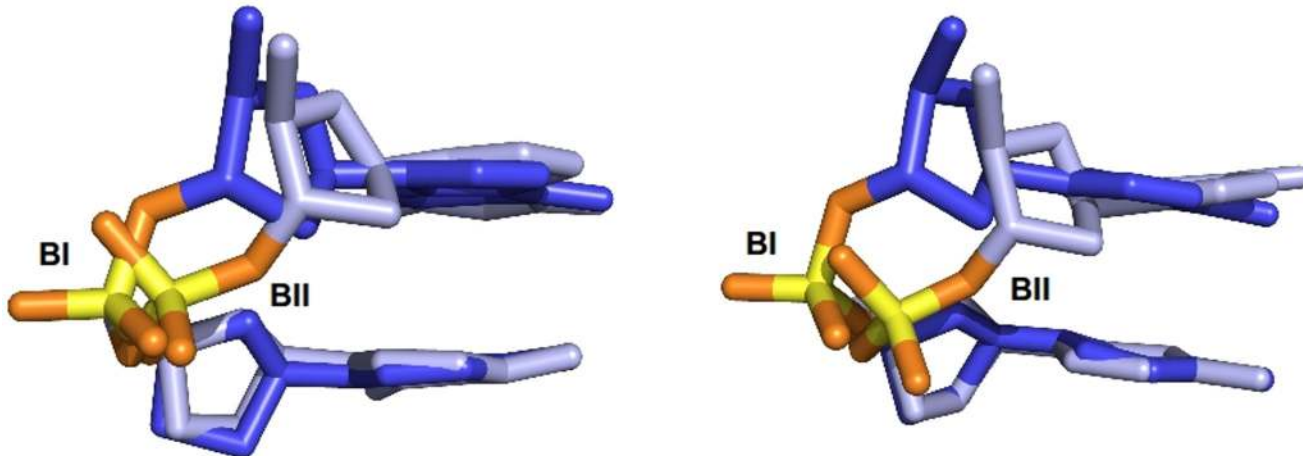
Fig 1. BI and BII conformations in the B-DNA backbone. Illustration of the BI ( \langle \epsilon\text{-}\zeta \rangle = -90^\circ ) and BII ( \langle \epsilon\text{-}\zeta \rangle = +100^\circ ) phosphate linkage conformations with a GpC dinucleotide extracted from MDs carried out with the Parmbsc0 _{\epsilon\zeta\text{OL1}} (left) or CHARMM36 (right) force fields.
