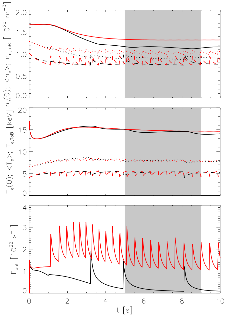
Figure 13. Same as figure 7 for the case where main ion density at the separatrix was increased from 4 to 5.3 \cdot 10^{19} \text{ m}^{-3} and electron and ion temperature was decreased from 800 to 500 \text{ eV} .
