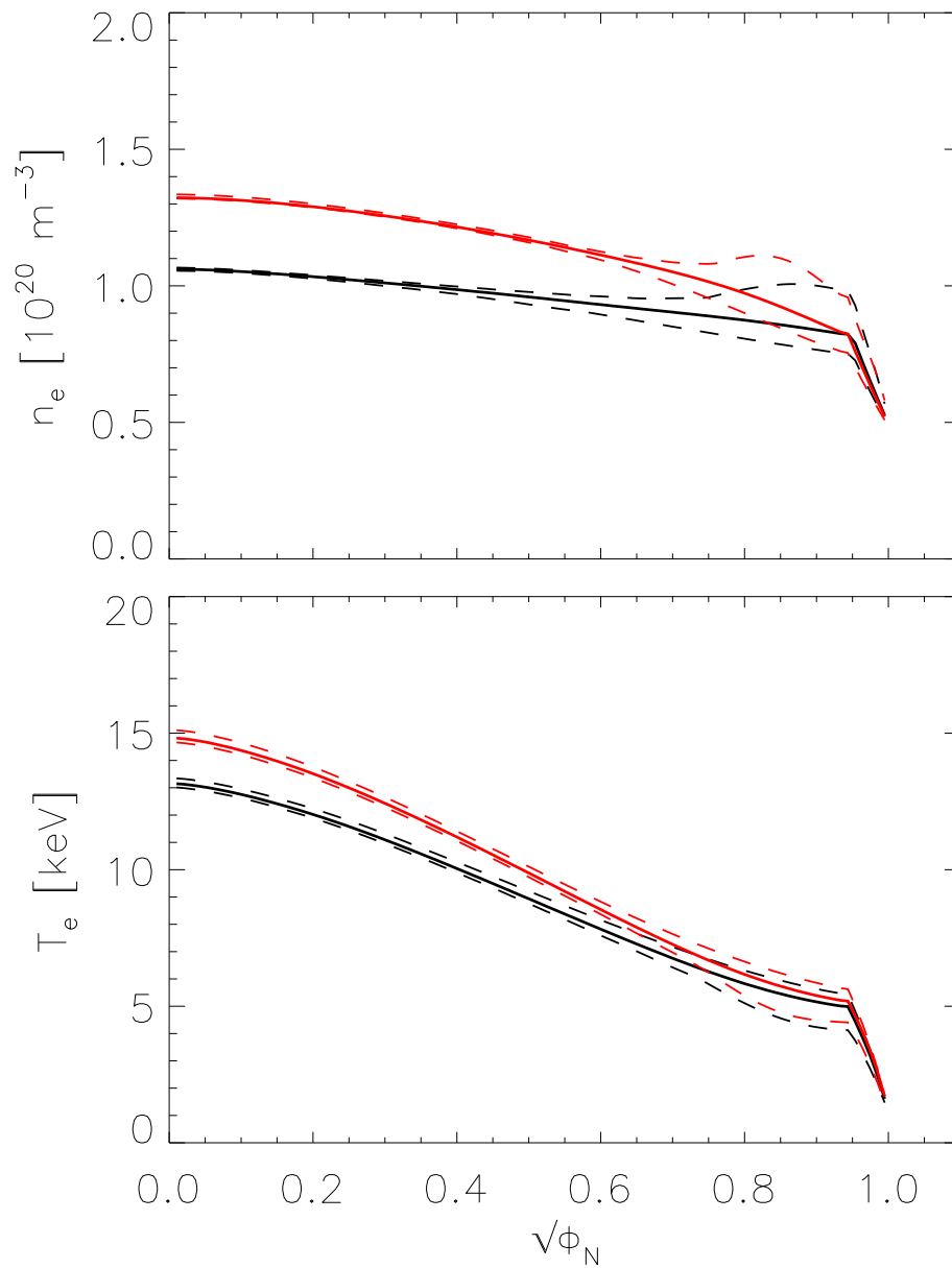
Figure 8. Same as figure 6 for the case where the Bohm/gyro-Bohm particle diffusivity was increased by a factor of three in the region affected by the pellet ablation. The red lines correspond to the base case and are shown for comparison.
