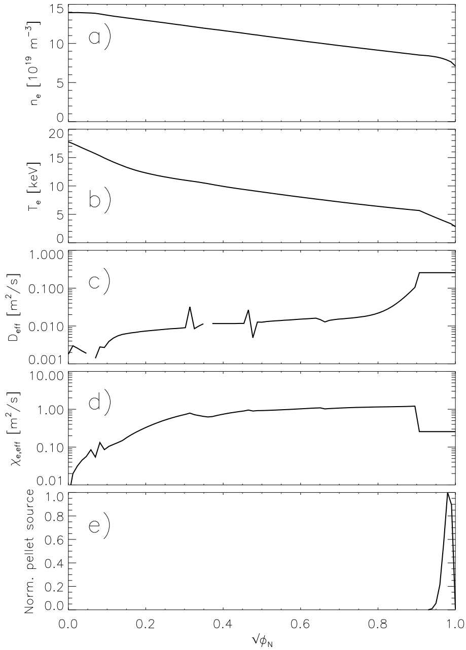
Figure 3. Simulation of a pellet fuelled ITER scenario 2 plasma with ASTRA equipped with the GLF23 transport model, continuous ELMs and continuous pellets. a) electron density profile, b) electron temperature profile, c) effective particle diffusivity, d) effective electron thermal conductivity, e) normalized pellet particle source.
