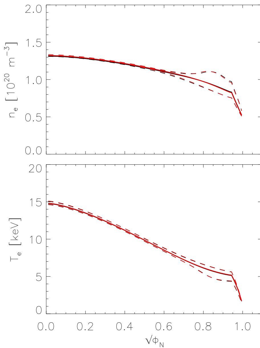
Figure 12. Same as figure 8 for the case where the recycling factor R was increased from 0 to 0.2.
