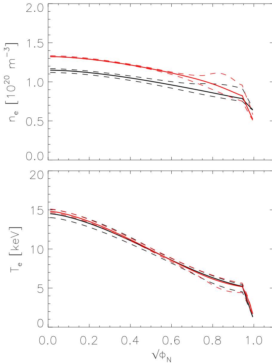
Figure 14. Same as figure 8 for the case where main ion density at the separatrix was increased from 4 to 5.3 \cdot 10^{19} \text{ m}^{-3} and electron and ion temperature was decreased from 800 to 500 \text{ eV} .
