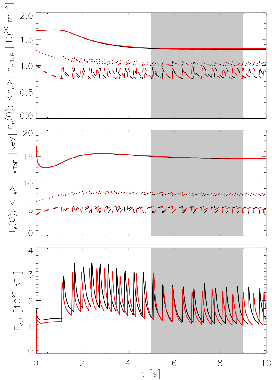
Figure 11. Same as figure 7 for the case where the recycling factor R was increased from 0 to 0.2.
