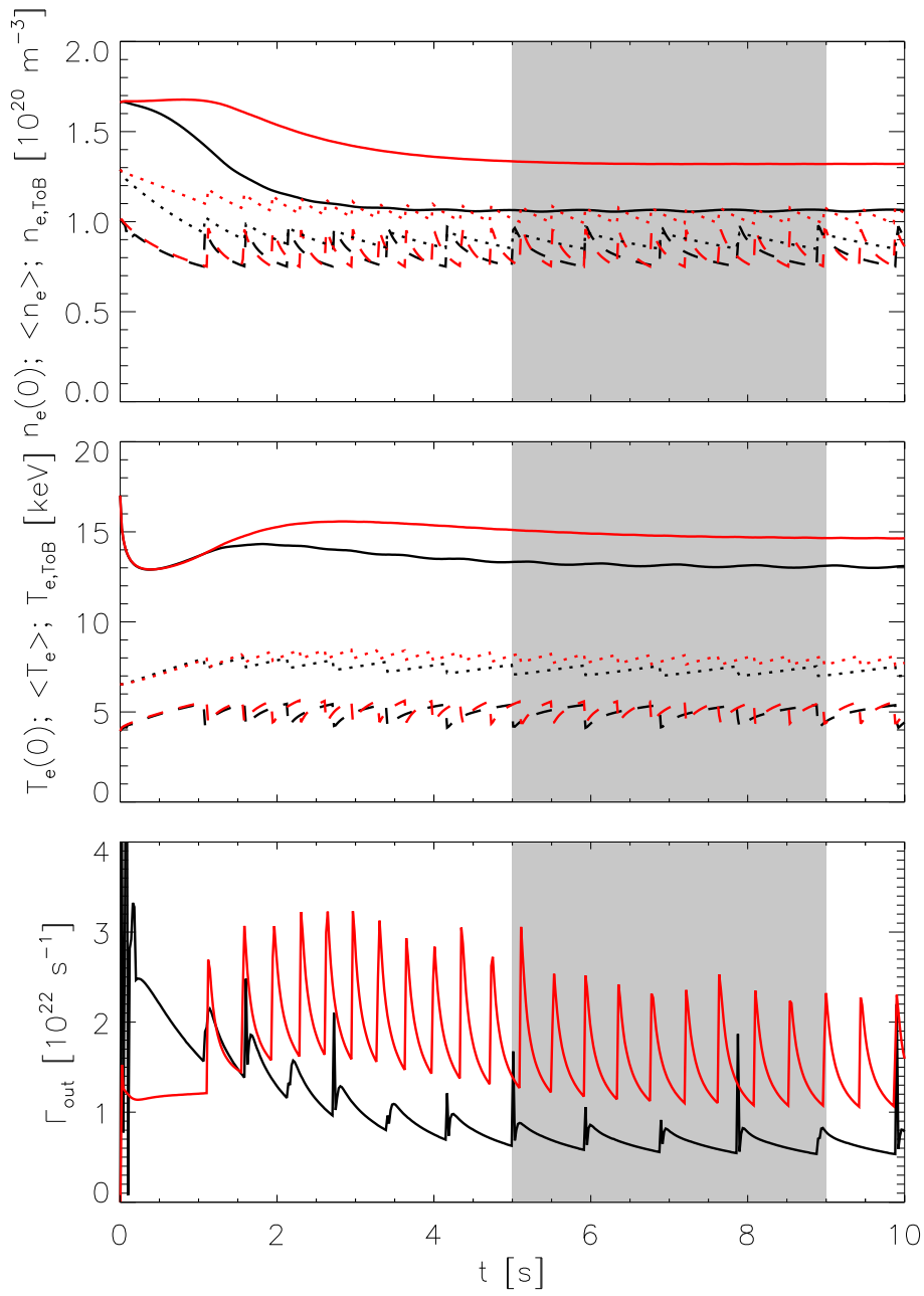
Figure 7. Same as figure 5 for the case where the Bohm/gyro-Bohm particle diffusivity was increased by a factor of three in the region affected by the pellet ablation. The red lines correspond to the base case and are shown for comparison.
