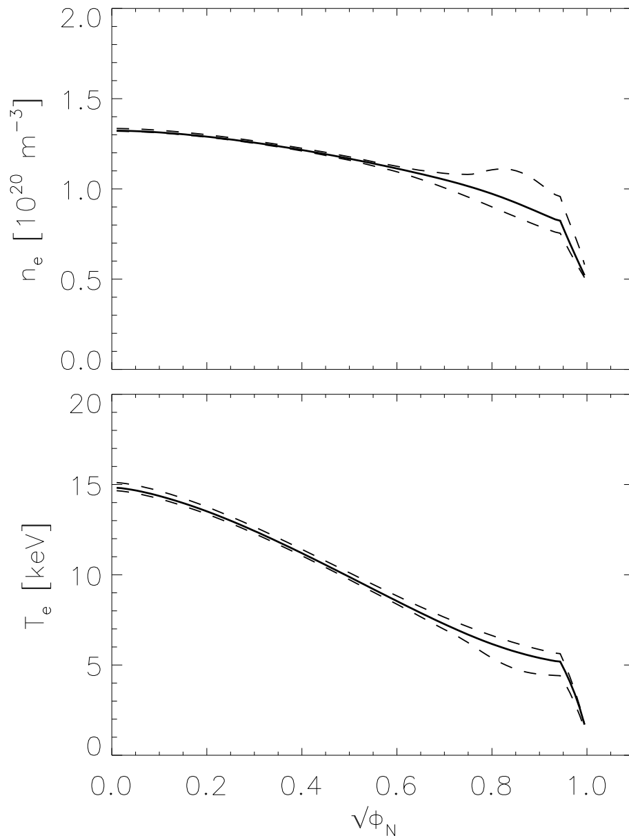
Figure 6. Electron density (top) and temperature profiles for the reference simulation of the ITER pellet fuelled baseline scenario. Solid lines indicate profiles averaged over the time window highlighted in 5 and dashed lines show the extremes between which the profiles oscillate between two successive pellet injections.
