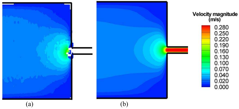
Figure 16. Velocity magnitude contour plots at the center plane ( y = 0 ) near the contraction at Q = 1 ml/h for the geometry used in the experiments ( w_c = 26 \mu\text{m} , h = 55 \mu\text{m} ). (a) Experimental results; (b) Numerical predictions.
