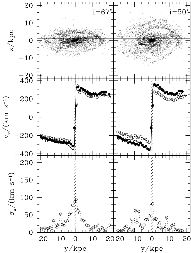
FIG. 10.—Rotation curve of the gas component of the simulated galaxy, estimated from the kinematics of gas measured in a 2 kpc-wide slit aligned with the major axis of the gas distribution. The panels of the left and right columns correspond to inclinations of 67^\circ and 50^\circ , respectively. The top panels show the distribution of gas particles. The mean velocity and dispersion across the slit are shown with open circles in the middle and bottom panels, respectively. The filled circles in the middle panels correspond to the circular velocity inferred from these kinematic data after correcting for inclination and asymmetric drift. After this correction, the inferred circular velocities agree well with the true circular speed (solid line), implying that the gas component is on a thin, centrifugally supported disk with a well-behaved velocity field. [See the electronic edition of the Journal for a color version of this figure.]
