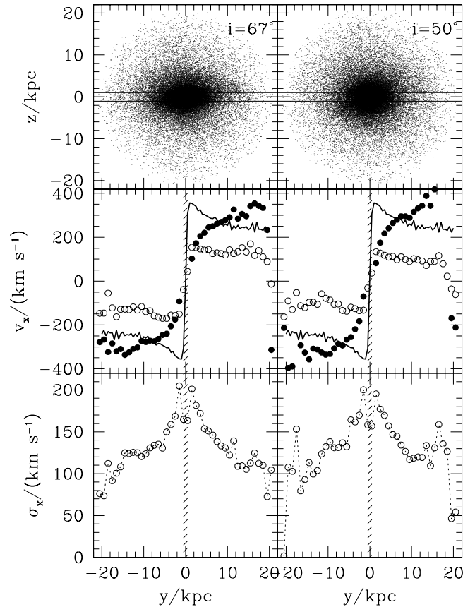
FIG. 11.—Same as Fig. 10, but for the stellar component. The velocity dispersion in the stars is comparable to the mean rotation speed at most radii, making it difficult to estimate circular speeds from single-slit kinematic information. Indeed, even after correcting for asymmetric drift and inclination, there is poor agreement between inferred (filled circles) and true (solid line) circular velocities. [See the electronic edition of the Journal for a color version of this figure.]
