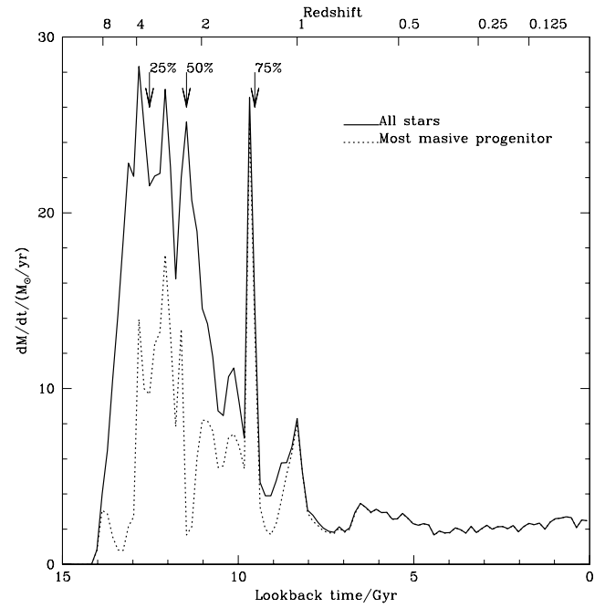
FIG. 5.—Distribution of stellar ages corresponding to stars identified within r_{\text{lum}} = 21 \text{ kpc} at z = 0 . Downward-pointing arrows indicate the formation times of the first 25%, 50%, and 75% of stars. Peaks in the distribution are easily traced to major merger events between progenitors of the final galaxy, the last of which happens at z \sim 1 . Afterward, the star formation rate stabilizes at around \sim 2 M_{\odot} \text{ yr}^{-1} , which corresponds roughly to the rate of smooth accretion of cooled gas within the luminous radius of the galaxy. The dotted line corresponds to the stars formed within the luminous radius of the most massive progenitor. About half of the stars formed earlier than z \sim 1.5 are formed in progenitors that are later merged within the final galaxy. [See the electronic edition of the Journal for a color version of this figure.]
