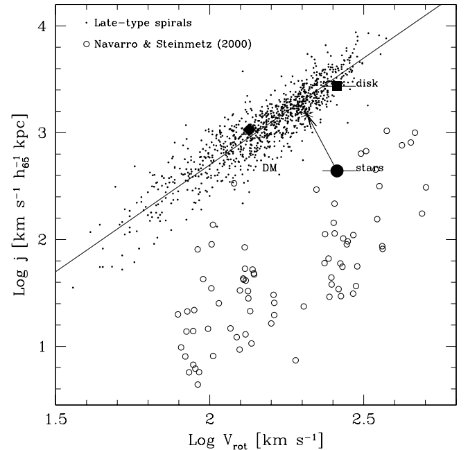
FIG. 12.—Rotation speed vs. specific angular momentum. The small filled circles correspond to late-type spirals taken mostly from the Tully-Fisher samples of Mathewson et al. (1992) and Courteau (1997), as compiled by Navarro (1998). The open circles correspond to the simulations of NS00b, which are similar to the one we present here but of lower resolution. We interpret the fact that the simulated galaxy is on the upper envelope of earlier simulations not as a result of improved numerical resolution but as mainly due to the particularly quiet assembly history of the halo under consideration. The location of the dark matter halo in this plane is shown by the filled diamond, assuming V_{\text{rot}} = V_{200} = 134 \text{ km s}^{-1} . The filled circle corresponds to the simulated galaxy, assuming that the rotation speed is that measured at R = 2.2R_d = 11 kpc. The solid square indicates the location of the disk component, computed adopting the same angular momentum estimator as applied to observed data, j = 2R_d V_{\text{rot}} . The agreement indicates that the size of the disk component is similar to that of late-type spirals of similar V_{\text{rot}} . The arrow points to where the simulated galaxy would be if the spheroidal component were removed, as discussed in the text. This confirms that the disk component of the simulated galaxy is structurally similar to observed late-type spirals. [See the electronic edition of the Journal for a color version of this figure.]
