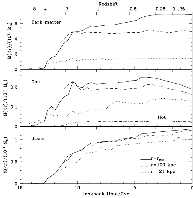
FIG. 4.—Evolution of the mass in the dark matter, gaseous, and stellar components within various radii. Solid lines indicate the mass within the virial radius r_{200} , dashed lines correspond to the mass within 100 physical kpc, and dotted lines to the mass within 21 physical kpc, which we define as the fiducial luminous radius of the galaxy at z = 0 . The line labeled “hot” in the gas panel corresponds to the total mass in the hot, diffuse component within r_{200} . [See the electronic edition of the Journal for a color version of this figure.]
