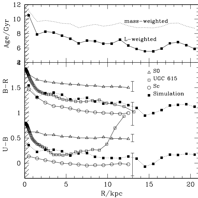
FIG. 7.— Top : Age profile of the stellar component of the simulated galaxy seen face-on. The filled squares indicate the luminosity-weighted age in circular radial bins; the dotted line corresponds to mass-weighted ages. Bottom : Color profiles of the simulated galaxy (filled squares) compared with Sab galaxy UGC 615 (open squares), as well as with the typical color profiles of S0 and Sc galaxies. The profiles shown correspond to the mean color of all S0 and Sc galaxies of brightness comparable (within 1 mag) to the simulated galaxies in the sample of Jansen et al. (2000). The spread in color for each type is indicated with a vertical error bar. The colors of the simulated galaxy are too blue to be consistent with an S0 and too red to be consistent with an average Sc. There is also a mild color gradient toward bluer colors in the outer regions consistent with the age gradient shown in the top panel. The shaded area highlights a radius corresponding to the gravitational softening scale length. [See the electronic edition of the Journal for a color version of this figure.]
