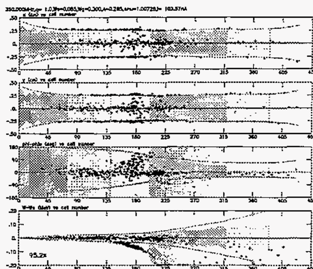
Figure 2. RFQTRAK simulated the LEDA RFQ using 100,000 macro particles. From top to bottom are: x, y, phase, and energy coordinates versus cell number. Bold-black points indicate lost particles. Only 10% of the lost particles are shown for clarity. The percentage transmission is 95.2%.
