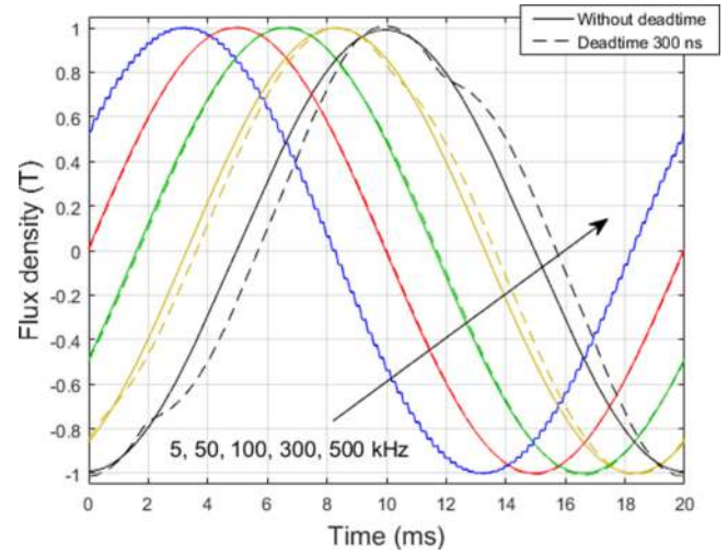
Fig. 12. Simulated flux-density waveforms at 5, 50, 100, 300, and 500 kHz switching frequencies both without and with deadtime when n = 3 .
