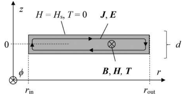
Fig. 7. Problem setting for the axisymmetric FE problem.
