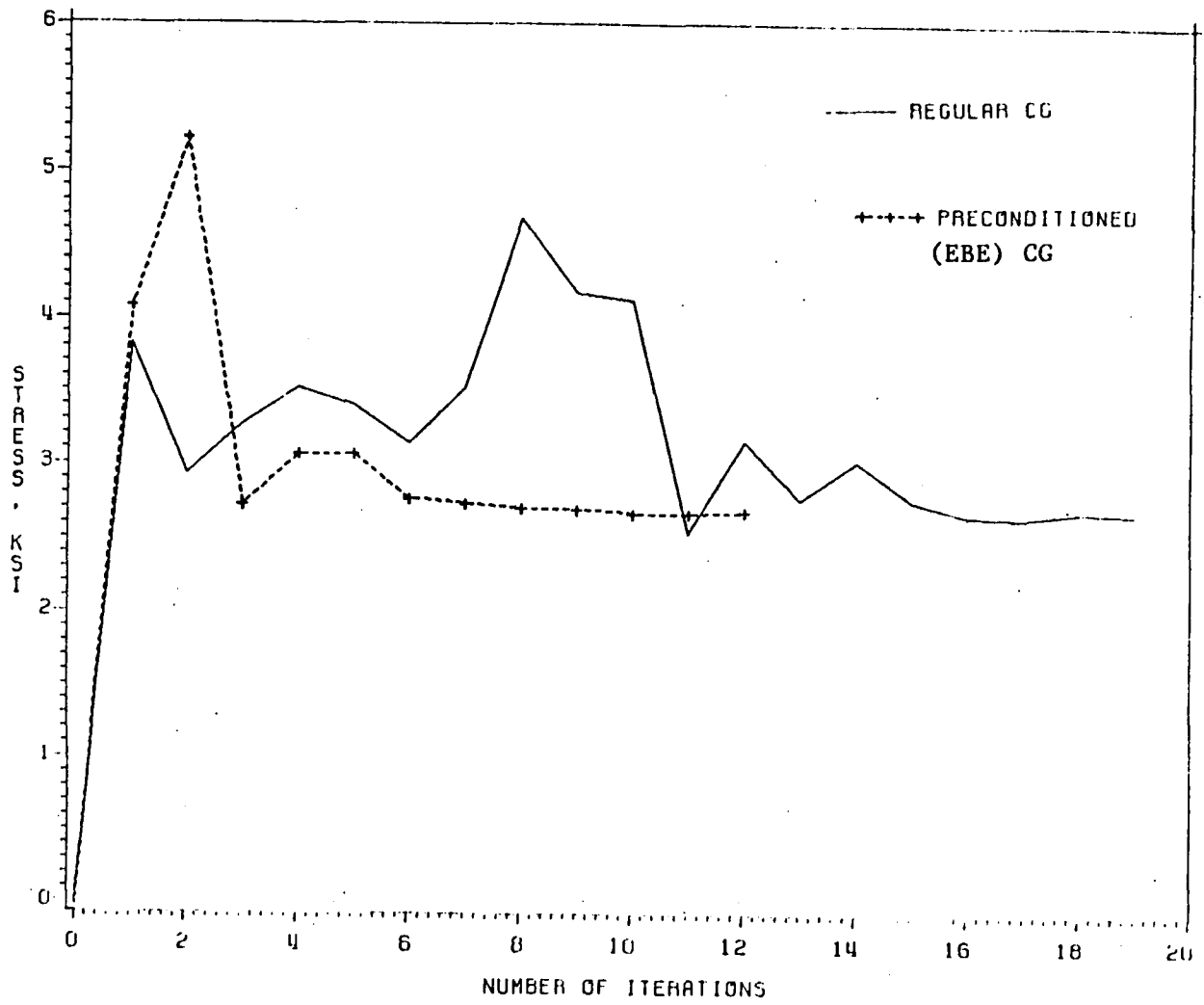
Figure 2: Convergence of Stress in Member 1 of 72-Bar Truss
