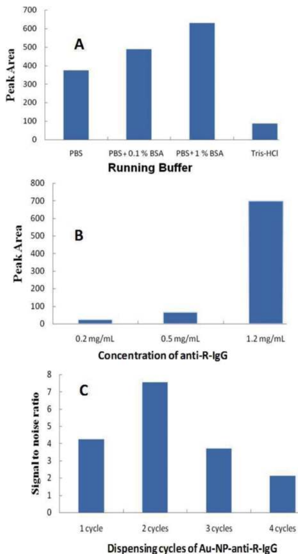
Fig. 3 Optimization of experimental parameters. (A) Effect of the running buffer constituents on the responses of LFD for the detection of R-IgG. Concentration of R-IgG in the sample solution: 100 ng mL -1 . The sample solutions were prepared with PBS (0.01 M, pH 7.0) containing 1% BSA. (B) Effect of the concentration of anti-R-IgG dispensed on the test zone on the response of the LFD for the detection of individual R-IgG. (C) Effect of the dispensing cycles of GNP-Ab on the conjugate pad on the response of the LFD for the detection of individual R-IgG. The anti-R-IgG solution with a concentration of 1.2 mg mL -1 was used to prepare the test line. The assay time: 7 min. The volume of the sample solution: 130 μL.
