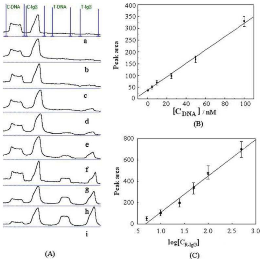
Fig. 4 Analytical performances of the LFD. (A) The typical responses of the LFD with increasing DNA and protein concentrations. From curve a to i, the concentrations of target DNA (nM) and IgG (ng mL -1 ) are 0, 1, 5, 10, 25, 50, 100, 500, 1000. (B) The resulting calibration curve of DNA test. (C) The resulting calibration curve of R-IgG test. Error bars represent standard deviation, n = 6 . Other conditions are the same as in Fig. 2.
