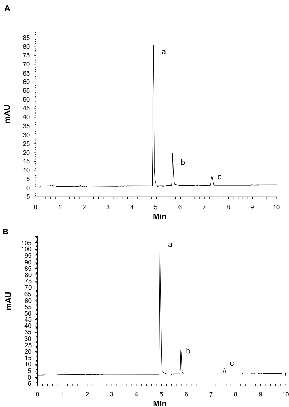
Figure 7. Application of the proposed method for the simultaneous determination of SG and MF in co-formulated tablets. (A) Janumet ® 50–500 tab. (a) MF: 311.3 \mu\text{g}/\text{mL} (b) IS: 40 \mu\text{g}/\text{mL} (c) SG: 40 \mu\text{g}/\text{mL} . (B) Janumet ® 50–1000 tab. (a) MF: 466.9 \mu\text{g}/\text{mL} (b) IS: 40 \mu\text{g}/\text{mL} (c) SG: 40 \mu\text{g}/\text{mL} .
