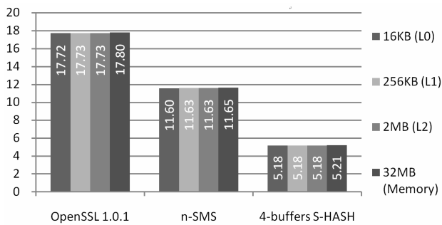
Figure 2. SHA-256 hashing from different cache levels and memory, Intel® Core™ i5-2500 (Architecture Codename Sandy Bridge). The performance of the 4-buffers SHA-256 S-HASH is compared to the (standard) serial hashing with the OpenSSL 1.0.1 implementation, and to the n -SMS method (see explanation in the text).
