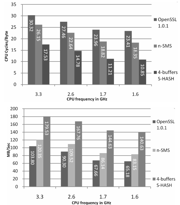
Figure 3. Hashing the files in the directory DIVERSE (see explanation in the text). Measurements are taken on the Core i5-2500, operating at different CPU frequencies. Panel a shows the performance in Cycles per Byte. Panel b shows the performance in MB/sec.
