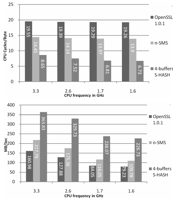
Figure 4. Hashing the files in the directory UNIFORM (see explanation in the text). Measurements are taken on the Core i5-2500 operating at different CPU frequencies. Panel a shows the performance in Cycles per Byte. Panel b shows the performance in MB/sec.
