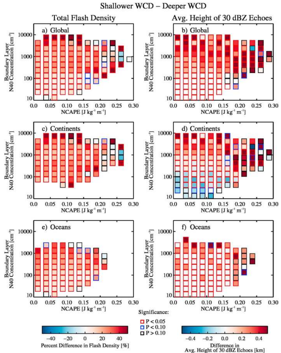
Figure 9. (left) Differences in total lightning density (TLD) and (right) the average height of 30 dBZ echoes (AVGHT30) between shallower WCD ( \text{WCD} < 4200 \text{ m} ) and deeper WCD ( \text{WCD} > 4200 \text{ m} ) for (a and b) the global population of LPCFs and CFs, (c and d) LPCFs and CFs over continents, and (e and f) LPCFs and CFs over oceans for a fixed NCAPE/N40 point. Shading indicates the percent difference in total lightning density and the difference in AVGHT30 in the left and right panels, respectively. Colored outlines for each point in the two-dimensional parameter space illustrate the significance of the difference determined by a Wilcoxon rank-sum test for the difference of medians. CFs (LPCFs) with \text{AVGHT30} > 5 \text{ km} (with flash rates above the minimum detection threshold of the TRMM lightning imaging sensor) were analyzed (both constraints in the case of LPCFs).
