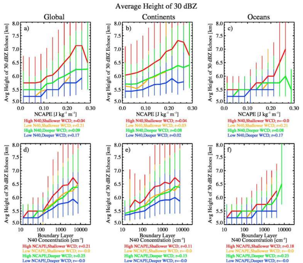
Figure 8. As in Figure 7 but for the partial sensitivity of the average height of 30 dBZ echoes (AVGHT30). CFs with AVGHT30 >5 km were analyzed. A threshold of 20 CFs was set for a given bin before the output was plotted.
