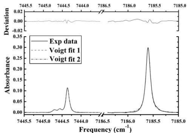
Fig. 4. Illustration of fitting of the absorption features.
