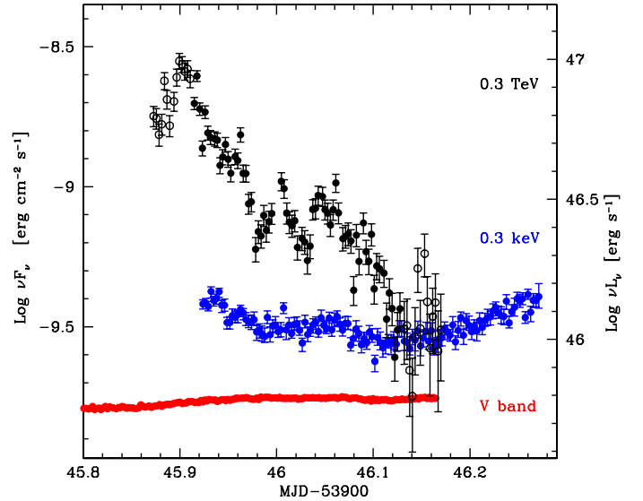
Fig. 3. Light curves of the \nu F_\nu flux at 0.3 TeV, 0.3 keV, and 5500 Å in 4-minute bins, plotted on the same flux scale. The right axis reports the corresponding luminosity scale. Note the remarkable difference of the amplitudes and the dramatic evolution in the VHE/X-ray flux ratio. HESS data (black): filled circles are fluxes calculated from the T300 light curve (integrated above threshold); empty circles from the T500 light curve (see text). The 0.3 TeV fluxes are corrected for intergalactic \gamma - \gamma absorption with a low-density EBL model, while both X-ray and optical fluxes are corrected for Galactic extinction ( A_V=0.071 ).
