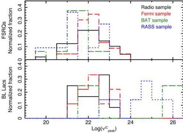
Fig. 18. The rest-frame inverse Compton \nu_{\text{peak}}^{\text{IC}} distributions of FSRQs and BL Lacs in different samples. Black solid histograms: radio sample; red dashed histograms: Fermi -LAT sample; green dot-dashed histograms: Swift BAT sample; blue dotted histograms: RASS sample.
