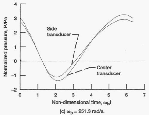
Figure 13.—Pressure variations at \theta = 337.5 deg.
