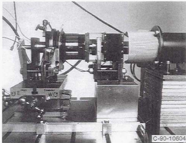
Figure 3.—A close-up view of the test rig.
