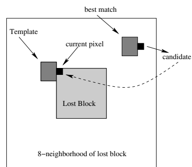
Figure 2: Basic texture synthesis procedure
